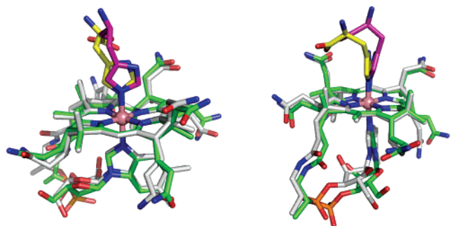
Figure 4. Two approximately perpendicular views of the superposition of one conformer of HisCbl with one of the B_{12} moieties present in the monoclinic structure of bovine TC (PDB entry, 2BB6). The B_{12} trunks are shown in white (HisCbl) and green (TC). The histidine residues are shown in yellow and magenta (His-175 in TC).
