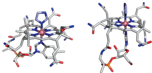
Figure 2. Two approximately perpendicular views of the molecular structure of ImCbl in a stick representation. The central Co atom is depicted as a pink sphere. N, O, and P atoms are drawn in blue, red, and orange, respectively. C atoms are drawn in gray in the B 12 trunk and in light blue in the \beta -ligand (imidazole conformation with higher occupancy). H atoms have been omitted for clarity. The figure was prepared using the program PyMol ( http://www.pymol.org/ ).
