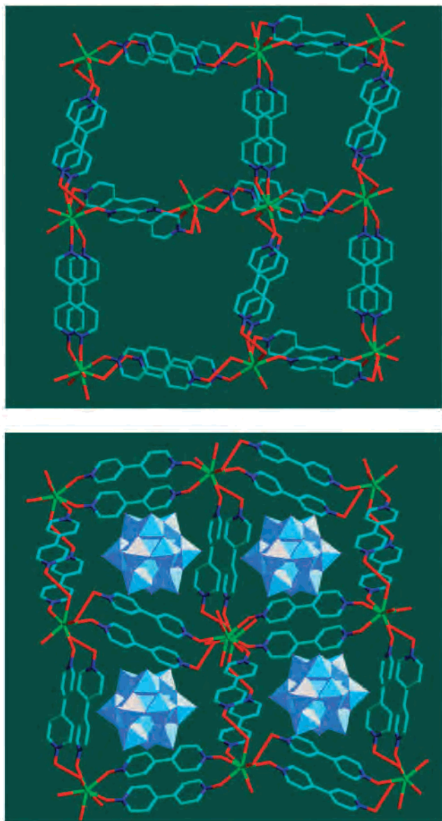
Figure 2. 3D 6^4 net formed by the [\text{Gd}(\text{dpdo})_4(\text{H}_2\text{O})_3]^{3+} units in compound 2 (top) and the 3D noninterwoven framework with distorted-honeycomb cavities occupied by the polyanions (bottom). Hydrogen atoms and the lattice solvent molecules are omitted for clarity.
