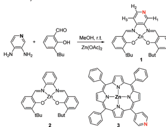
Scheme 1. Synthesis of Zn II -salen Derivative 1
