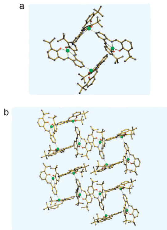
Figure 1. (a) X-ray solid-state structure of [ 1 ] 4 . Numbering scheme, H-atoms, and disordered cocrystallized toluene molecules have been omitted for clarity. (b) Parallel alignment of [ 1 ] 4 assemblies in the solid state, giving rise to channel formation along the crystallographic b axis.
