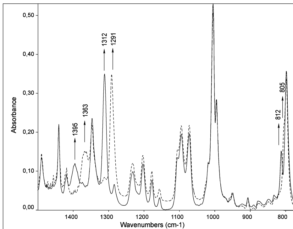
Figure 2. FTIR spectra of Fe(TPP)(NO 2 )(1Me-Im) (solid line) and Fe(TPP)( 15 NO 2 )(1-MeIm) (dashed line) obtained by the interaction of 1-MeIm vapors (~0,1 Torr) with thin layers containing Fe(TPP)(ONO) and Fe(TPP)(O 15 NO).
