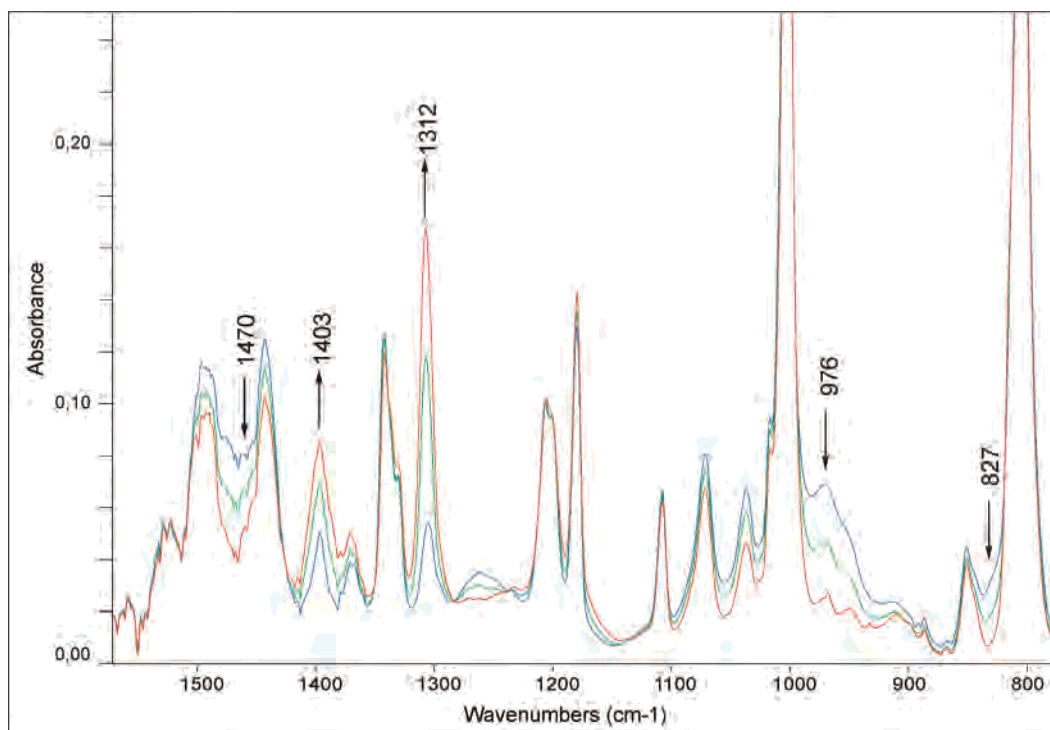
Figure 5. FTIR spectral changes observed in a sublimed layer of Fe(TTP)(ONO) in the presence of 1 Torr equivalent of NH 3 upon warming from 150 (blue) to 170 (green) and 200 K (red) and removal of excess NH 3 .
