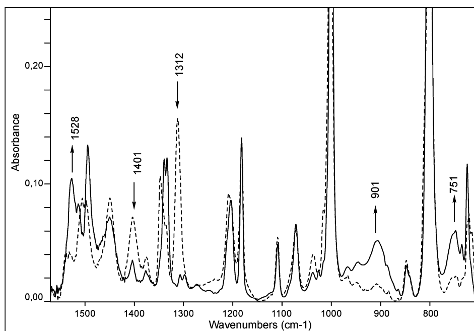
Figure 6. FTIR spectra of the ammine–nitro complex Fe(TTP)(NH 3 )(NO 2 ) (dashed line) after warming from 240 to 293 K upon intense pumping.
