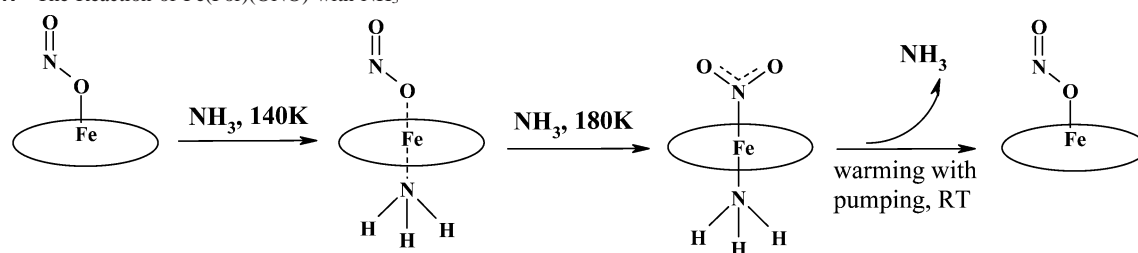
Scheme 1. The Reaction of Fe(Por)(ONO) with NH 3
