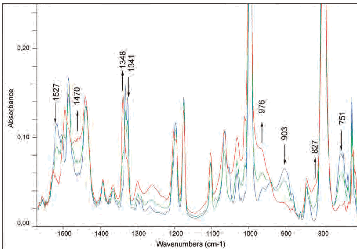
Figure 3. FTIR spectral changes observed for a sublimed layer of Fe(TTP)(ONO) (blue) after introducing 1 Torr equivalent of NH 3 into the cryostat at 77 K and while warming from 130 (green) to 150 K (red).
