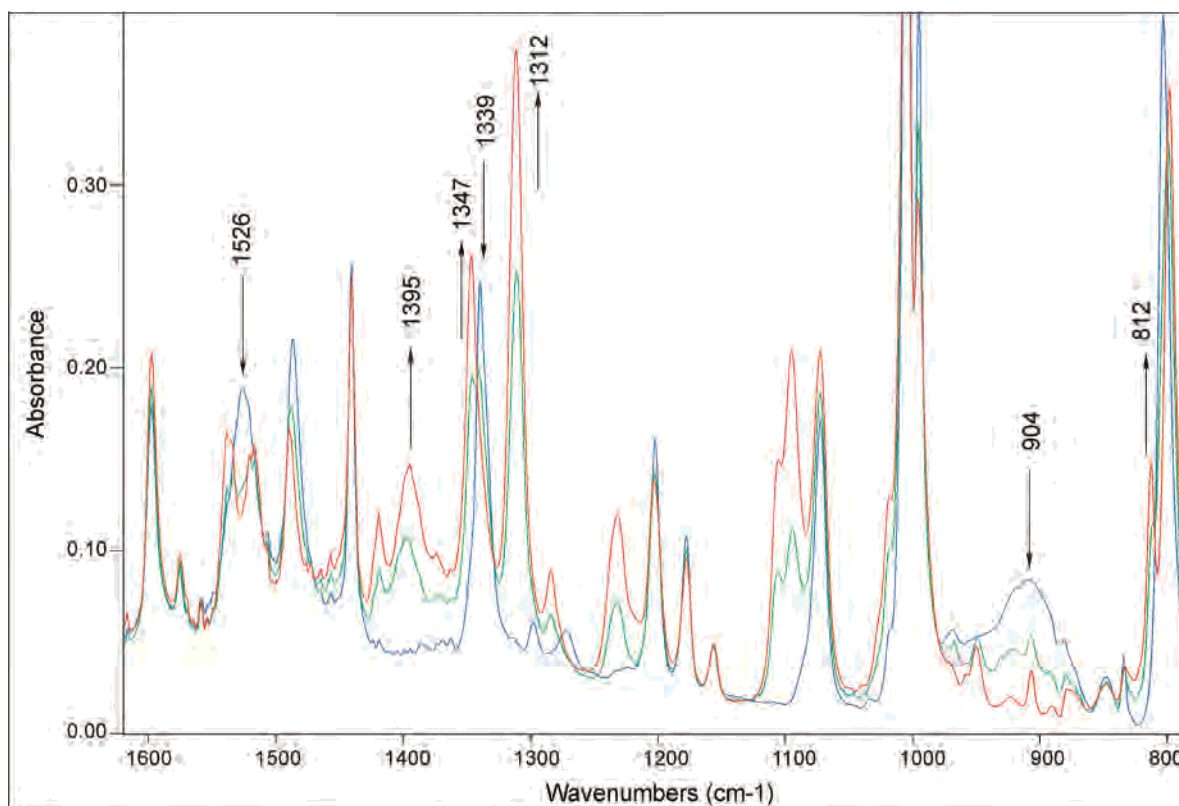
Figure 1. FTIR spectral changes observed in sublimed layers of Fe(TPP)(ONO) (blue) after supplying into cryostat \sim 0,1 Torr 1-Melm and subsequent measurements after 2 (green) and 5 (red) min.
