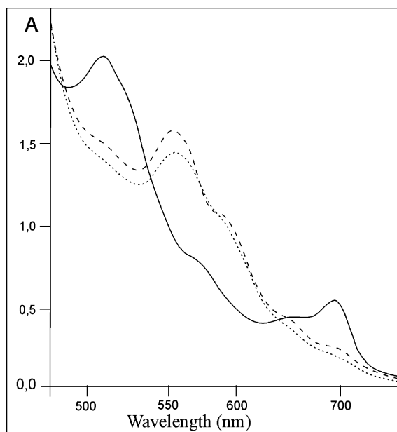
Figure 4. Optical spectra of Fe(TTP)(ONO) (solid line), Fe(TTP)(NH 3 )(ONO) (dashed line), and Fe(TTP)(NH 3 )(NO 2 ) (dotted line).
