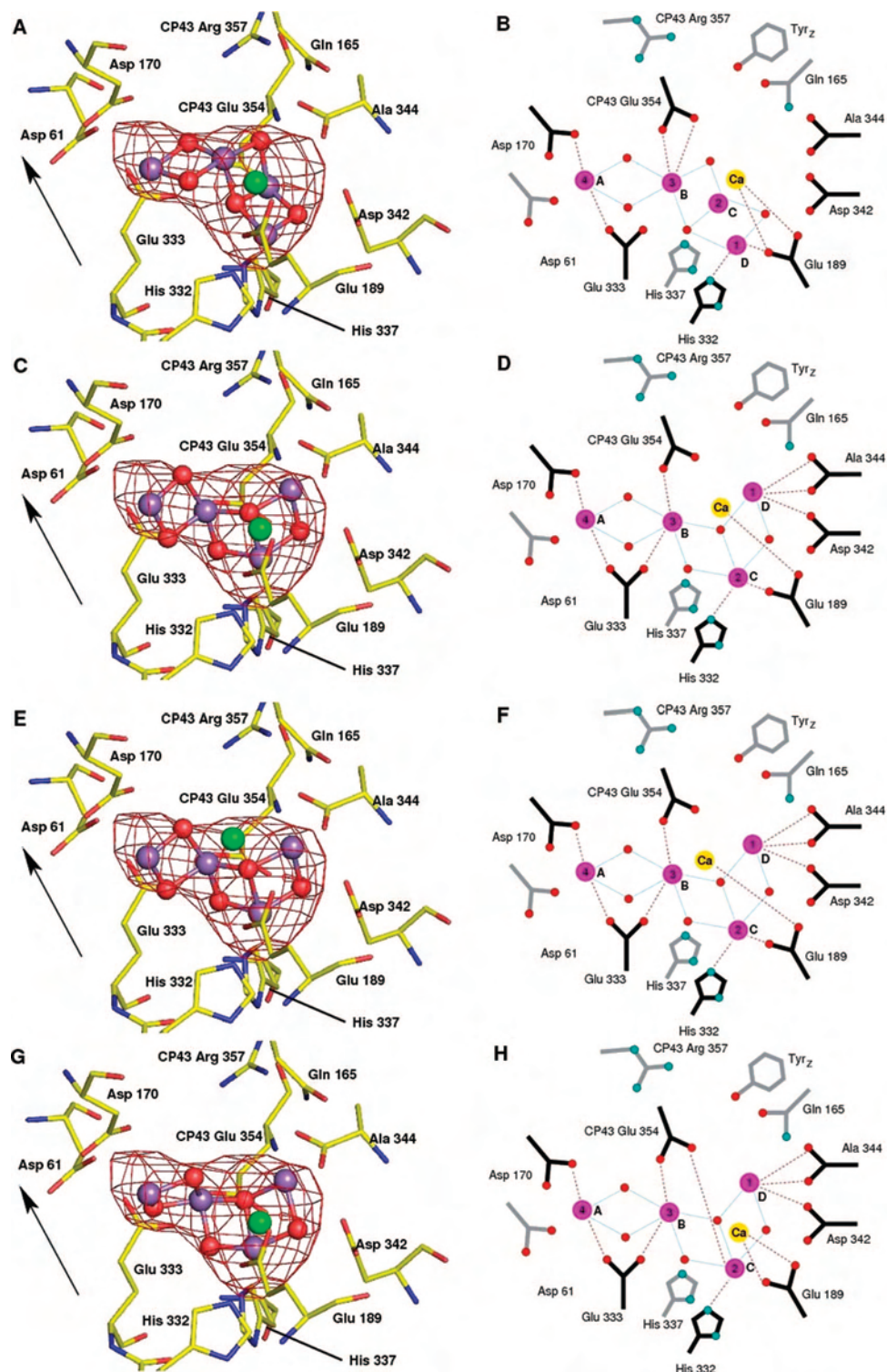
Figure 6. Refinement of the positioning of the EXAFS models (models I, II, IIa, and III) of Yano et al. 72 into the Mn-anomalous diffraction data of Ferreira et al. 7 by Barber and Murray. 71 Each EXAFS models were fitted by real-space refinement against the Mn-anomalous difference map of Ferreira et al. 7 using the molecular graphics program Coot . 87 The Mn-anomalous difference map is shown in red and contoured at 5\sigma . Parts A, C, E, and G are for EXAFS models I, II, IIa, and III, respectively, while parts B, D, F, and H are the schematic for each showing potential ligation patterns, where the lines are for distances of 2.8 Å or less. The arrows indicate the direction of the normal to the membrane plane.
