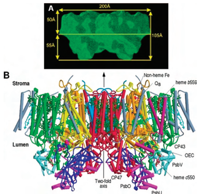
Figure 1. Side view of the PSII dimer isolated from T. elongatus viewed perpendicular to the membrane normal derived from (a) electron cryomicroscopy and single-particle analysis in the absence of negative staining at a resolution of about 20 Å (Duncan, J.; Nield, J.; Barber, J., unpublished) and (b) X-ray crystallography at a resolution of 3.5 Å. 7 For the X-ray structure, helices are represented as cylinders with D1 in yellow, D2 in orange, CP47 in red, CP43 in green, Cyt b559 in wine red, PsbL, PsbM, and PsbT in medium blue, and PsbH, PsbI, PsbJ, PsbK, PsbX, PsbZ, and Ycf12 in gray. 22 The extrinsic proteins are PsbO in blue, PsbU in magenta, and PsbV in cyan. Chlorophylls of the D1/D2 RC are light green, Pheo's are blue, chlorophylls of the antenna complexes are dark green, \beta -carotenes are in orange, hemes are in red, nonheme Fe is red, and Q_A and Q_B are magenta. The oxygen-evolving centers (OEC) where water-splitting catalysis occurs is shown in red (O atoms), magenta (Mn ions), and cyan ( Ca^{2+} ) balls.
