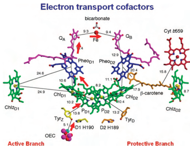
Figure 2. Cofactors involved in electron-transfer visualized perpendicular to the internal pseudo-two-fold axis. 7 The coloring scheme is the same as that in Figure 1. The phytol tails of the chlorophylls and Pheos have been removed for clarity. The side chains of Tyr Z (D1 Tyr161) and D1 His190 are shown in yellow and those of Y D (D2 Tyr160) and D2 His189 in orange. The four chlorophylls comprising P680 are in direct van der Waals contact. The electron-transfer pathway is indicated by red arrows, and distances are given in angstroms. Excitation of the RC, via light absorption by chlorophylls (Chl) in the antenna, drives electron transfer from the cluster of four chlorophylls bound to the D1 and D2 proteins to the Pheo acceptor, leading to the radical pair P680 + Pheo - . The radical cation of P is localized on P D1 , although the primary electron charge separation probably occurs from Chl D1 followed by hole migration, 29–31 while the radical anion is located on Pheo D1 . The electron on Pheo D1 - is rapidly donated to a firmly bound PQ Q A (shown in purple) and then transferred to a second PQ Q B (also shown in purple). This electron transfer is aided by the presence of a nonheme Fe located midway between them. When the PQ Q B is fully reduced and protonated to plastoquinol (PQH 2 ), it diffuses from the Q B binding site into the lipid matrix of the membrane. On the electron donor side, P680 + is reduced by a redox-active tyrosine (Tyr Z ), which then extracts electrons from the Mn 4 CaO 4 cluster that constitutes the oxygen-evolving center (OEC). These electron-transfer processes occur mainly on the D1 side of the RC, and the symmetrically related cofactors located on the D2 side (Chl D2 and Pheo D2 ) are nonfunctional in primary charge separation. Other cofactors shown, including the heme of cytochrome b559 (Cyt b559 shown in red) and the \beta -carotene molecule (shown in brown), play a role in protecting PSII against photoinduced damage. 11–14
