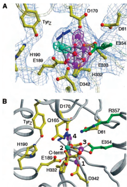
Figure 3. Structure of the water-splitting site from Ferreira et al. 7 view of the metal cluster (A) with side-chain ligands and (B) with possible catalytically important side-chain residues. Mn ions, Ca 2+ , and O atoms are shown in magenta, cyan, and red, respectively. One unidentified nonprotein ligand to the OEC and modeled as carbonate is colored in blue. The protein main chain is depicted in light gray, while the side-chain bonds and C atoms follow the coloring of the protein subunits (D1, yellow; CP43, green). In part A, the \sigma_A -weighted 2|F_o| - |F_c| density is shown as a light-blue wire mesh contoured at 1.5\sigma . Anomalous difference Fourier maps at 1.89340 Å (Mn edge, contoured at 10\sigma ) and 2.25430 Å (highlights Ca 2+ , contoured at 7\sigma ) wavelengths are shown in magenta and blue-green, respectively.
