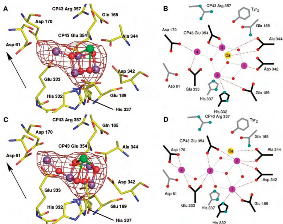
Figure 5. Two models of the catalytic site of the OEC based on X-ray crystallography. (A) The Mn_4Ca cluster as proposed by Ferreira et al. 7 positioned within the Mn-anomalous difference map of Ferreira et al. 7 with amino acid side chains. (B) Schematic representation of the amino acid ligation pattern for the model in part A with a distance of less than 2.8 Å shown by connecting lines. (C) Remodeling the OEC by Barber and Murray 70 using the native electron-density maps of Ferreira et al. 7 and Loll et al. 8 and the Mn-anomalous difference map of Ferreira et al., 7 keeping the Mn_3CaO_4 cubane of Ferreira et al. but with Mn4 (dangler Mn) linked to it via a single 3.3 Å mono- \mu -oxo bridge. (D) Schematic representation of the amino acid ligation pattern for the model in part C with a distance of less than 2.8 Å shown by connecting lines. The Mn-anomalous difference map is shown in red and contoured at 5\sigma . The arrow indicates the direction of the normal to the membrane plane. The fitting of the models for the metal cluster was performed by real-space refinement using the molecular graphics program Coot . 87
