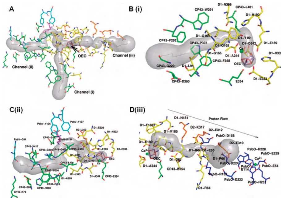
Figure 4. Identification of three channels leading from the OEC to the luminal side of PSII. 60 (A) All three channels identified by analyses using the program CAVER. 91 (B) Details of channel i suggested to be a route for oxygen to diffuse from the OEC. (C) Details of channel ii, which could act as a proton/water channel for the OEC. (D) Details of channel iii, which has been identified previously as a likely proton/water channel for the OEC. 7,92 The Ca 2+ binding site on the PsbO protein 59 is also shown. Amino acid residues within 4 Å of the center of the pathway are shown in a stick representation and are color-coded to their respective proteins as follows: D1, yellow; CP43, green; D2, orange; PsbV, cyan; PsbU, magenta. Modified from Murray and Barber. 60
