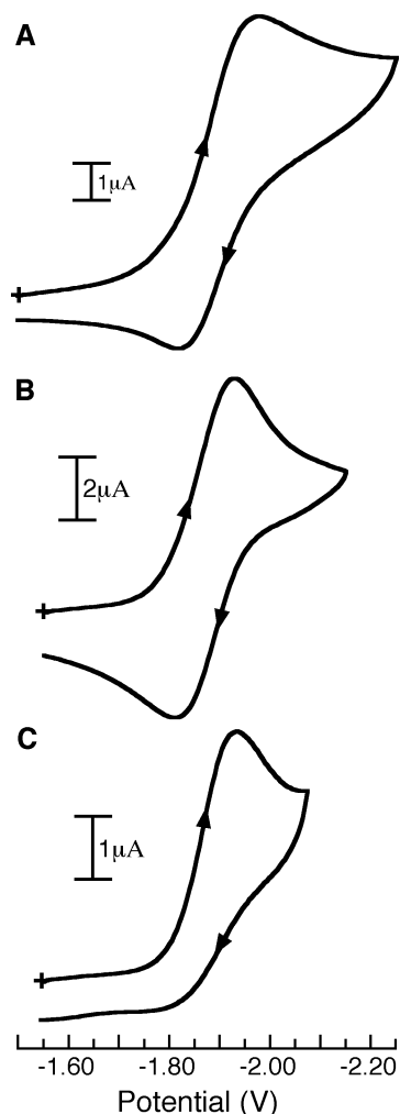
Figure 4. CVs of [\text{Fe}^{\text{III}}\text{H}_2\text{2ipr}(\text{OH})]^- (A), [\text{Fe}^{\text{III}}\text{H1ipr}(\text{OH})]^- (B), and [\text{Fe}^{\text{III}}\text{0ipr}(\text{OH})]^- (C) recorded as DMA solutions and referenced versus [\text{Cp}_2\text{Fe}]^{0/+} .
