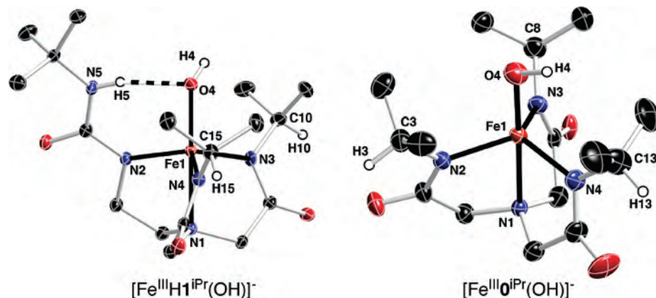
Figure 2. Thermal ellipsoid plots illustrating the molecular structures of [\text{Fe}^{\text{III}}\text{H1}^{\text{iPr}}(\text{OH})]^- and [\text{Fe}^{\text{III}}\text{0}^{\text{iPr}}(\text{OH})]^- . Thermal ellipsoids are drawn at the 50% level, and for clarity only urea and methine hydrogen atoms are shown. Only one of the disorder fragments containing N3 is shown for [\text{Fe}^{\text{III}}\text{H1}^{\text{iPr}}(\text{OH})]^- .
