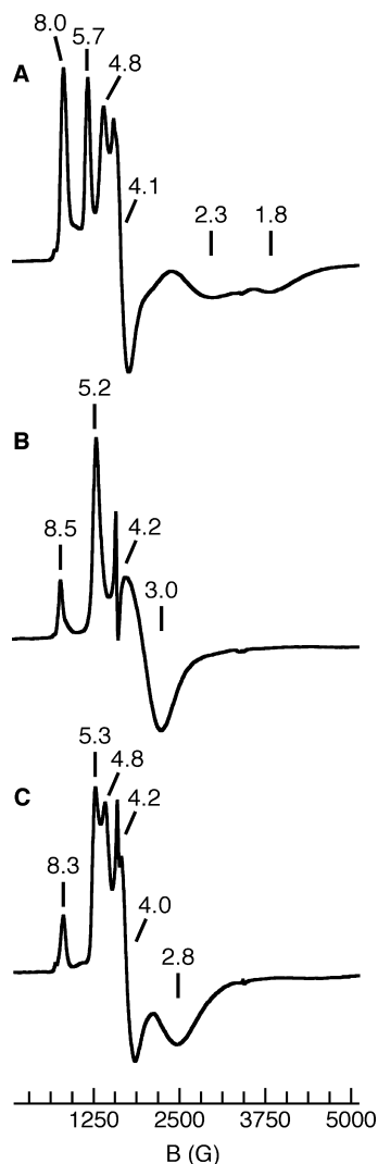
Figure 3. X-band EPR spectra of [\text{Fe}^{\text{III}}\text{H}_2\text{2}^{\text{iPr}}(\text{OH})]^- (A), [\text{Fe}^{\text{III}}\text{H1}^{\text{iPr}}(\text{OH})]^- (B), and [\text{Fe}^{\text{III}}\text{0}^{\text{iPr}}(\text{OH})]^- (C) recorded as DMA solutions at 4 K.
