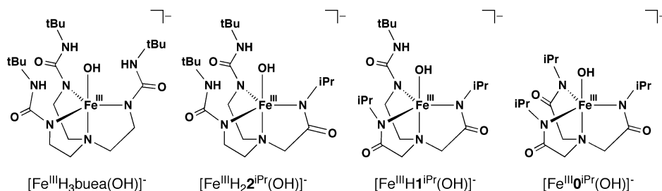
Figure 1. Fe III OH complexes with varied H-bond networks used in this study.
