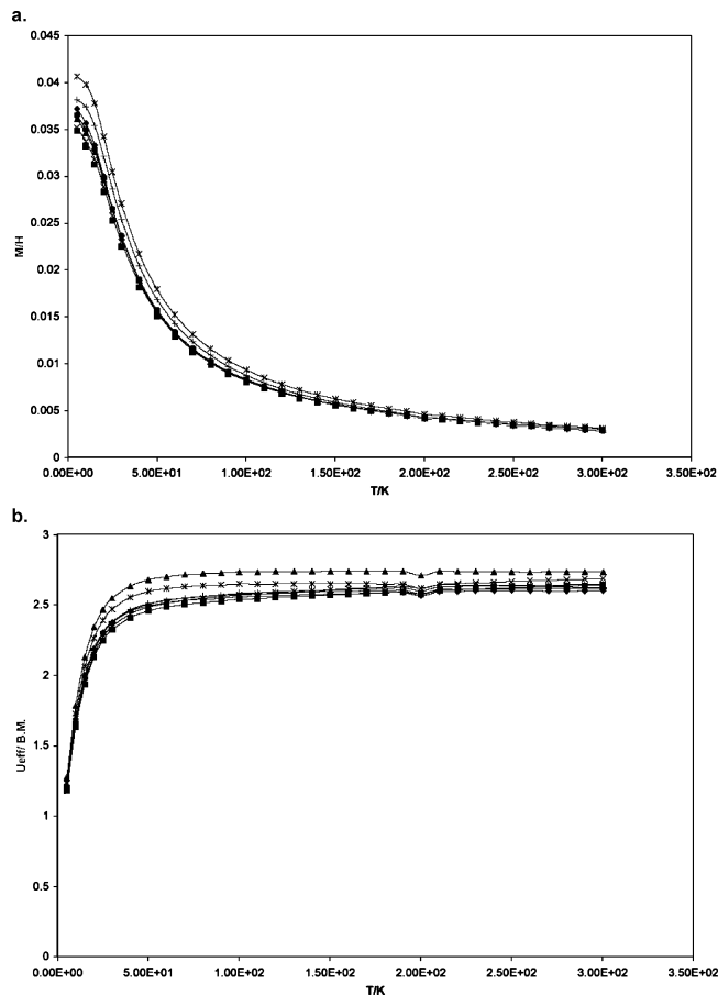
Figure 5. a. M/H vs T plots for (\text{silox})_3\text{MoEt} ( 2-MoEt ) generated from 7 runs using 3 different samples. b. \mu_{\text{eff}} vs T plots for 2-MoEt corresponding to those in a.
