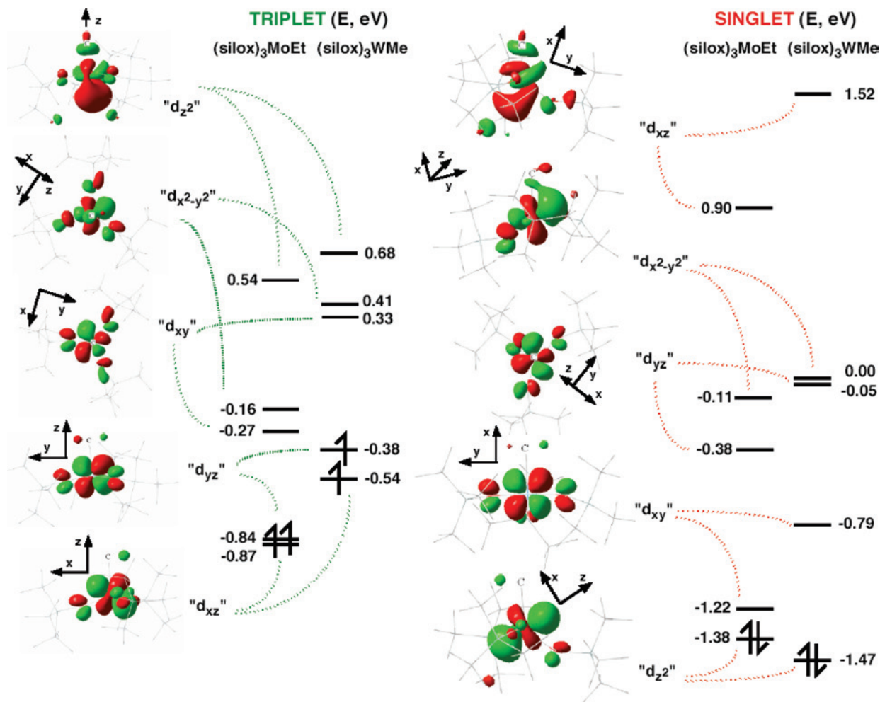
Figure 7. Orbitals (red and green) and their energies (1 eV = 8065.5 cm -1 ) of triplet and singlet (silox) 3 MR (MR = MoEt, 2-MoEt; WMe, 2-WMe). Orbitals shown for the triplets are those of 2-MoEt; those of 2-WMe are very similar. Orbitals shown for the singlets are those of 2-WMe; those of 2-MoEt are very similar.
