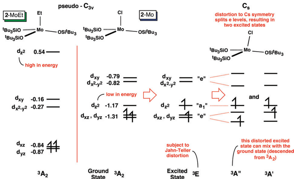
Figure 8. The low-lying d_{z^2} orbital in (\text{silox})_3\text{MoCl} (2-Mo) suggests that low-lying excited states derived from an (e)^1(a_1)^1 configuration (i.e., (d_{xz})(d_{yz})(d_{z^2})^1 ) in C_{3v} should Jahn–Teller distort to C_s symmetry; mixing of the appropriated excited-state with the {}^3A_2 ground state (GS) of 2-Mo ( C_{3v} ) provides the means for the observed GS distortion (Renner–Teller).
