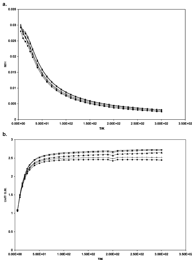
Figure 4. (a) M/H vs T plots for (\text{silox})_3\text{MoCl} ( 2-Cl ) generated from 5 runs using 3 different samples. (b) \mu_{\text{eff}} vs T plots for 2-Cl corresponding to those in a.
