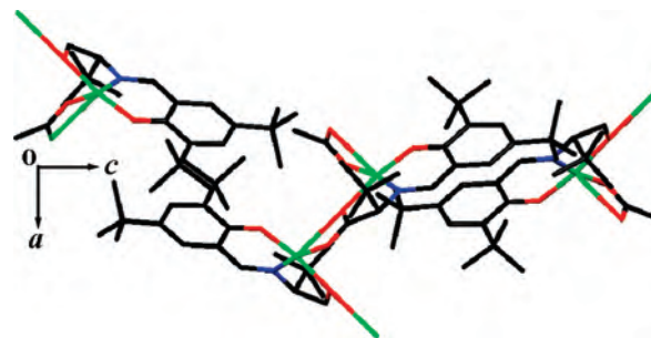
Figure 2. Crystal packing of 1a .
