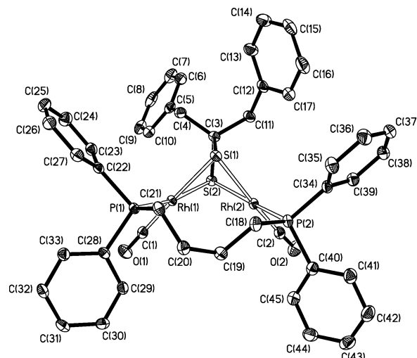
Figure 7. Molecular structure of [\text{Rh}_2(\mu\text{-S}_2\text{CBn}_2)(\text{CO})_2(\mu\text{-dppb})] ( 16 ). no)butane), resulted in the formation of cis disubstituted complexes. The reaction of 7 with 1 mol equiv of dppb gave a yellow solution of the compound [\text{Rh}_2(\mu\text{-S}_2\text{CBn}_2)(\text{CO})_2(\mu\text{-dppb})] ( 16 ), which was isolated as a yellow solid in good yield. The structure of 16 has been determined by X-ray diffraction methods and is shown in Figure 7. The spectroscopic data obtained from the IR and NMR are in agreement with an approximate C_3 molecular symmetry as a result of the coordination of the diphosphine in a cis fashion. The diastereotopic >\text{CH}_2 protons of the benzyl groups of the bridging gem-dithiolato ligand are isochronous in \text{C}_6\text{D}_6 and gave a single resonance at 3.94 ppm in the ^1\text{H} NMR spectrum. However, the spectrum in \text{CDCl}_3 showed the expected AB quartet centered at 3.56 ppm ( J_{\text{AB}} \approx 14 Hz). The ^{31}\text{P}\{^1\text{H}\} NMR spectrum features a slightly broad doublet with no fine structure centered at 32.25 ppm ( J_{\text{Rh-P}} = 157 Hz). Finally, the equivalent carbonyl ligands were observed as a broad absorption at 1980\text{ cm}^{-1} in the IR spectrum in dichloromethane.
