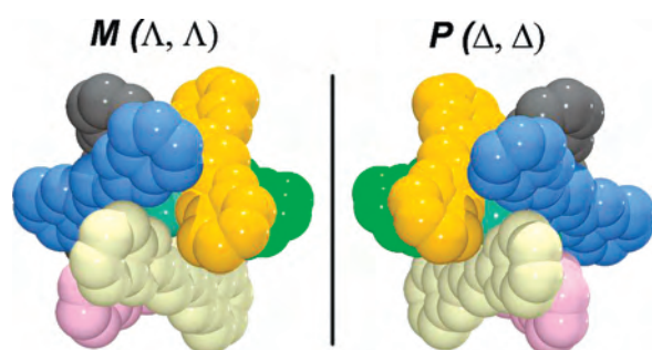
Figure 5. Space-filling representation of the two enantiomers present in 1 viewed down the C_3 axis. For clarity hydrogen atoms are omitted and each \text{H}_2\text{L}^- ligand is represented in a different color, with zinc ions are represented by dark-green color.
