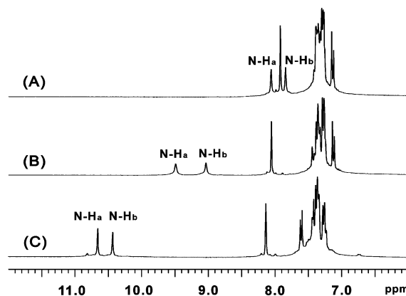
Figure 1. Binding of \text{Cl}^- in complex 2·BF 4 monitored by ^1\text{H} NMR spectroscopy ( \text{CD}_2\text{Cl}_2 ): (A) a solution of 2·BF 4 ; (B) a solution of 2·BF 4 with 0.5 equiv of ^n\text{Bu}_4\text{NCl} ; (C) a solution of 2·BF 4 with 5.0 equiv of ^n\text{Bu}_4\text{NCl} .
