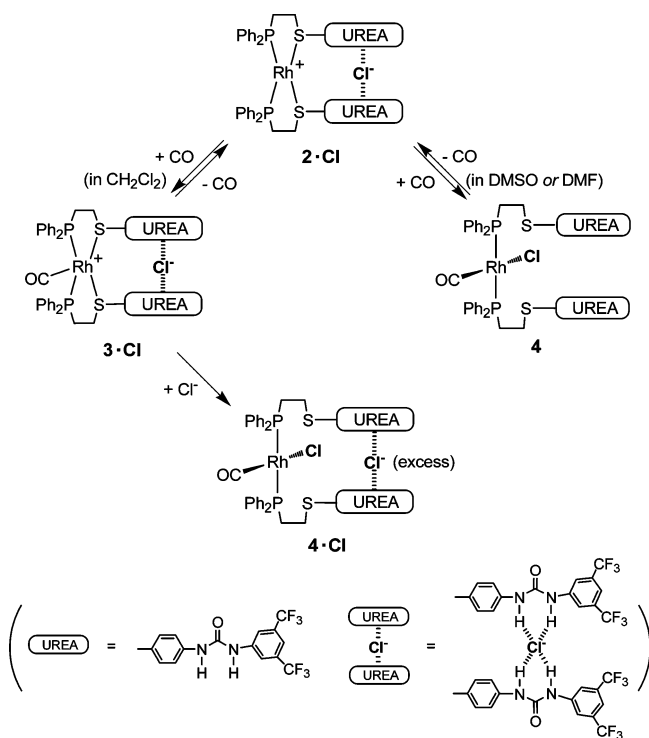
Scheme 1. Systematic Structural Changes of 2 \cdot \text{Cl} That Accompany the Addition and Removal of \text{CO}/\text{Cl}^-
