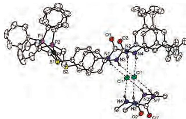
Figure 3. X-ray crystal structure of complex 2·Cl with thermal ellipsoids set at 50% probability. For clarity, all H atoms except those on the urea N atoms are omitted. Dotted lines indicate the intermolecular hydrogen-bonding interactions between the Cl atoms and the urea H atoms. Symmetry code: ' = 1 - x, 1 - y, -z.
