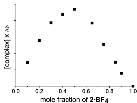
Figure 2. Job plot from the addition of ^n\text{Bu}_4\text{NCl} to the complex 2·BF 4 .
