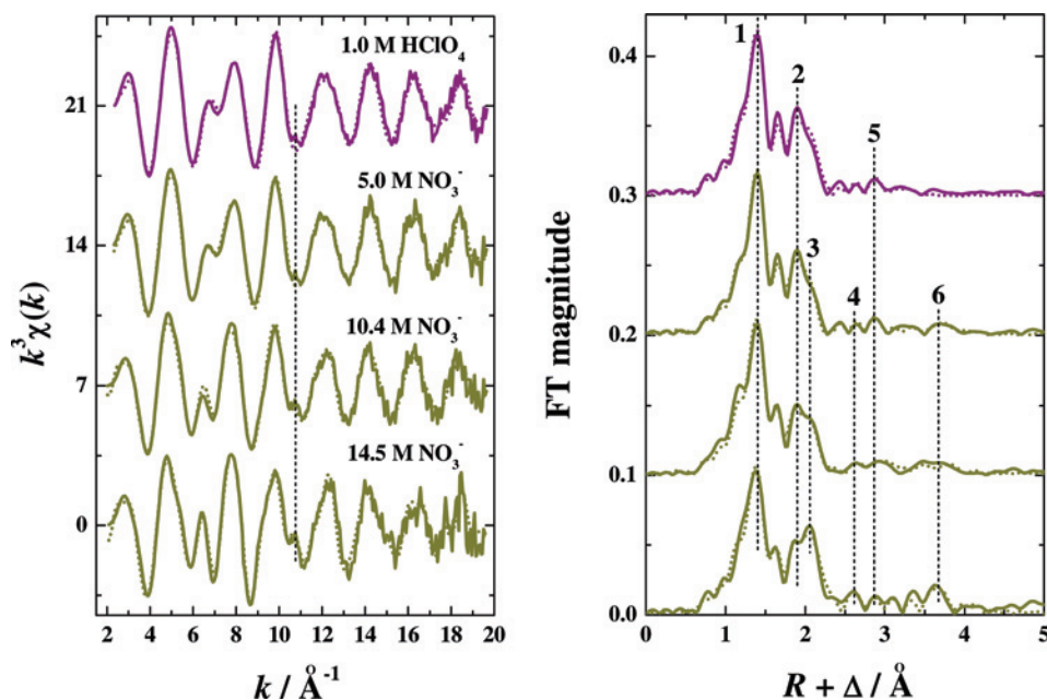
Figure 9. k^3 -weighted Np L_{III} -edge EXAFS spectra (left) and their corresponding FTs (right) for Np^{VI} in aqueous perchlorate and nitrate solutions: —, experimental data; ···, theoretical fit; FT range, k = 2.0 – 19.5 \text{ \AA}^{-1} ; phase shifts are not corrected on the FTs; solvent compositions, “5.0 M NO_3^- ” = 1.0 M HNO_3 /4.0 M NH_4NO_3 , “10.4 M NO_3^- ” = 4.4 M HNO_3 /6.0 M NH_4NO_3 , and “14.5 M NO_3^- ” = 14.5 M HNO_3 ; numbers of FT peaks, 1 = O_{ax} , 2 = O_{eq}(H_2O) , 3 = O_{eq-co}(NO_3) , 4 = N, 5 = O_{ax} MS, 6 = O_{dist}(NO_3) and its MS. The data color reflects the actual color of the sample solutions. The dotted line on the EXAFS spectra represents the [2p4f] double-electron excitation. See the text.
