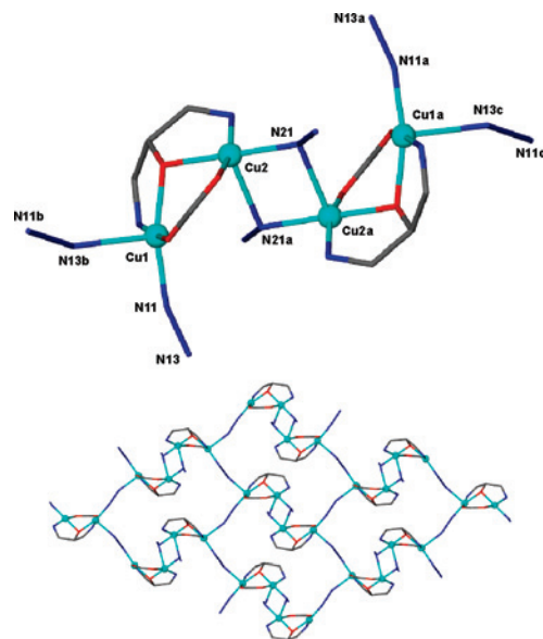
Figure 5. Assembly of two dinuclear units (top) of 3 and the 2D layer running along the (1, 0, -1) plane (bottom). Symmetry code: a, 2 - x , - y , - z ; b, 1.5 - x , 0.5 + y , 1.5 - z ; c, 0.5 + x , -0.5 - y , 0.5 + z . Color scheme as in Figure 1.
