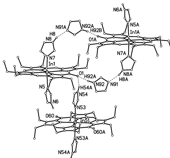
Figure 5. Drawing of the interactions between the hydrogen-bonded aggregate \{(im)_2In^{III}(OEPO\cdots im)\}_2 and the centrosymmetric (im)_2In^{III}(OEPO) molecule in \{(im)_2In^{III}(OEPO\cdots im)\}_2 \cdot (im)_2In^{III}(OEPO) \cdot 2Cl_2C_6H_4 . For clarity, atoms are represented by arbitrarily sized circles and the solvate molecules are not shown. Only those hydrogen atoms involved in hydrogen bonding are shown.
