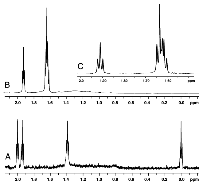
Figure 2. 1 H NMR spectra of the region of methyl resonances for (trace A) \{\text{In}^{\text{III}}(\text{OEPO})\}_2 in chloroform- d and (trace B) (\text{py})_2\text{In}^{\text{III}}(\text{OEPO}) formed by dissolving \{\text{In}^{\text{III}}(\text{OEPO})\}_2 in pyridine- d 5 . The inset (trace C) shows an expansion of the 2.0–1.5 ppm region of the spectrum in B.
