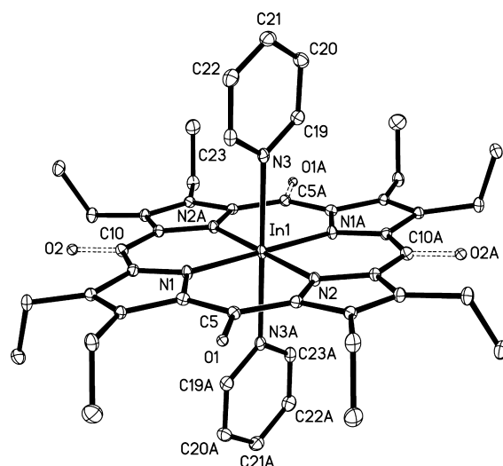
Figure 6. Drawing of the centrosymmetric (py)_2In^{III}(OEPO) molecule with 30% thermal contours. Selected bond distances (Å): In1–N1, 2.1203(18); In1–N2, 2.1204(18); In1–N3, 2.4065(19); C5–O1A, 1.293(5). Selected bond angles (deg): N1–In1–N3, 91.43(7); N2–In1–N3, 88.78(7).
