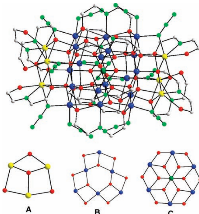
Figure 6. Molecular structure of the cation of 7 (top) and the three types of constituent layers of its core (bottom). Only the ipso -C atoms of the pdm 2- /pdmH - phenyl groups are shown. H atoms have been omitted for clarity. Color scheme: Mn II , yellow; Mn III , blue; Mn IV , olive; O, red; N, green; C, gray.
