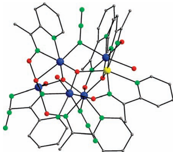
Figure 22. Molecular structure of the cation of complex 16 . H atoms have been omitted for clarity. Color scheme: Mn II , yellow; Mn III , blue; O, red; N, green; C, gray.
