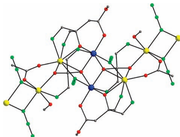
Figure 13. Molecular structure of complex 10 , with H atoms omitted for clarity. Color scheme: \text{Mn}^{\text{II}} , yellow; \text{Mn}^{\text{III}} , blue; O, red; N, green; C, gray.
