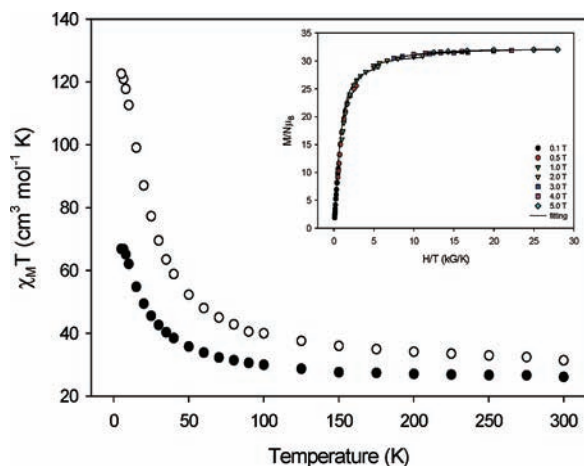
Figure 16. \chi_M T vs T plots for complexes 11 (●) and 12 (○) in a 1 kG field. Inset: Plot of M/N\mu_B vs H/T for 12 at the indicated fields. The solid lines are the fit of the data; see the text for the fit parameters.
