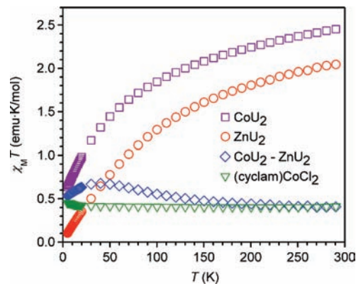
Figure 11. Variable-temperature magnetic susceptibility data for the trinuclear cluster (\text{cyclam})\text{Co}[(\mu\text{-Cl})\text{U}(\text{Me}_2\text{Pz})_4]_2 ( \text{CoU}_2 , purple squares) and (\text{cyclam})\text{Zn}[(\mu\text{-Cl})\text{U}(\text{Me}_2\text{Pz})_4]_2 ( \text{ZnU}_2 , red circles). 33 Blue diamonds correspond to a subtraction of the \text{ZnU}_2 data from the \text{CoU}_2 data. Magnetic data for the precursor complex (\text{cyclam})\text{CoCl}_2 are depicted as green triangles.
