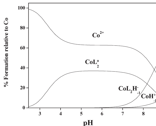
Figure 11. Speciation curves for complexes forming in the Co(II)–quinic acid system; c_{\text{Co}} = 0.001667\text{ mol dm}^{-3} , c_{\text{ligand}} = 0.006635\text{ mol dm}^{-3} . Charges are omitted for clarity.
