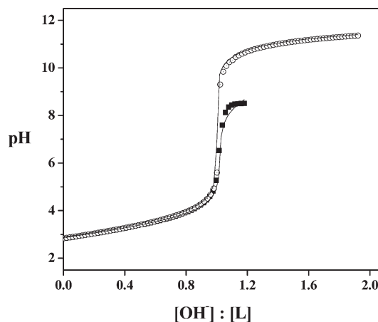
Figure 10. Potentiometric titration curves of free quinic acid (white circles; c_{\text{ligand}} = 0.004976 \text{ mol dm}^{-3} ) and Co(II)–quinic acid with molar ratios 1:3 (black squares); c_{\text{Co}} = 0.001639 \text{ mol dm}^{-3} , c_{\text{ligand}} = 0.004976 \text{ mol dm}^{-3} . Solid lines represent calculated curves.
