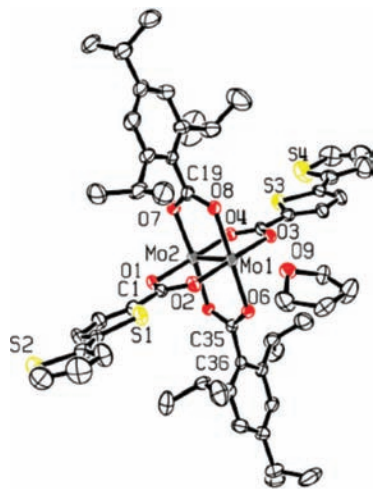
Figure 1. ORTEP drawing of the Mo 2 -bithienylcarboxylate complex. Reproduced with permission from ref 1. Copyright 2008 National Academy of Sciences.
