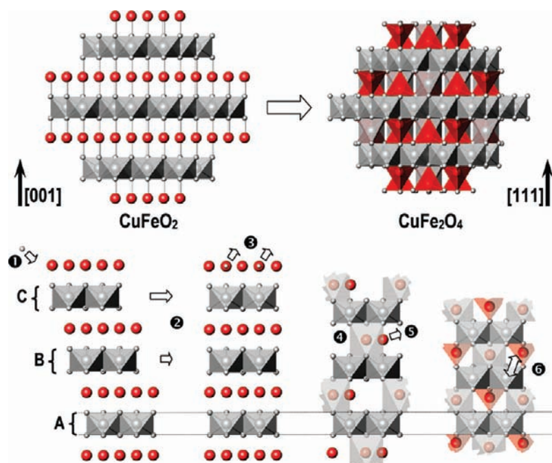
Figure 8. Schematic representation of the structural mechanism for the delafossite-to-spinel phase transition.
