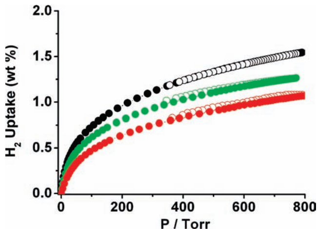
Figure 5. \text{H}_2 sorption isotherms of PCN-9s at 77 K (black symbol, Co; red symbol, Fe; green symbol, Mn; solid circle, adsorption; open circle, desorption).
