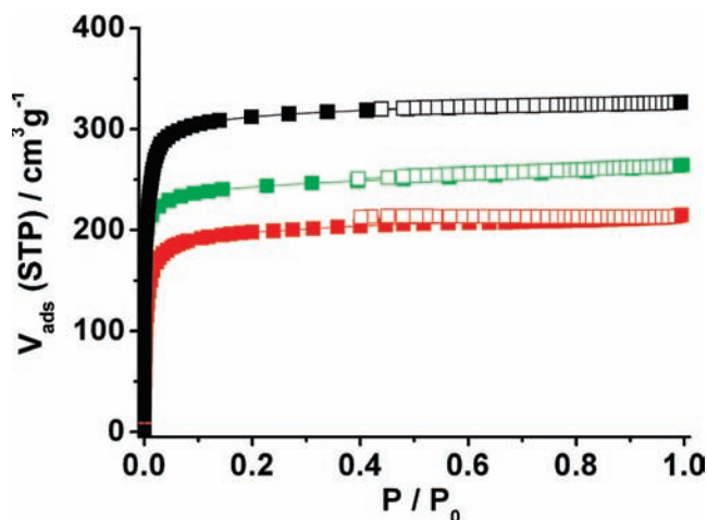
Figure 4. \text{N}_2 sorption isotherms of PCN-9s at 77 K (black symbol, Co; red symbol, Fe; green symbol, Mn; solid square, adsorption; open square, desorption).
