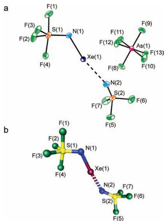
Figure 1. (a) The structural unit in the X-ray crystal structure of [\text{F}_4\text{S}=\text{N}-\text{Xe}\cdots\text{N}=\text{SF}_3][\text{AsF}_6] . Thermal ellipsoids are shown at the 50% probability level. (b) The gas-phase geometry of the \text{F}_4\text{S}=\text{N}-\text{Xe}\cdots\text{N}=\text{SF}_3^+ cation calculated at the MP2/aug-cc-pVTZ level of theory (Table 2).
