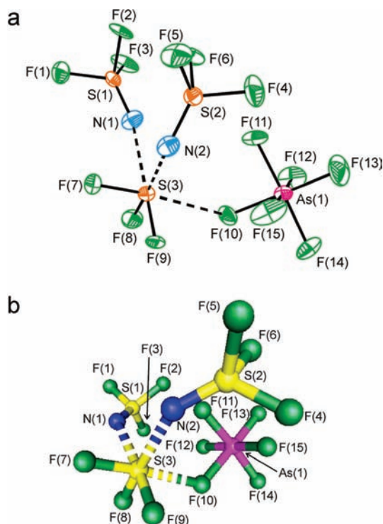
Figure 2. (a) The structural unit in the X-ray crystal structure of [\text{F}_3\text{S}(\text{N}=\text{SF}_3)_2][\text{AsF}_6] . Thermal ellipsoids are shown at the 50% probability level. (b) The gas-phase geometry of [\text{F}_3\text{S}(\text{N}=\text{SF}_3)_2][\text{AsF}_6] calculated at the PBE1PBE/aug-cc-pVTZ level of theory (Table 3).
