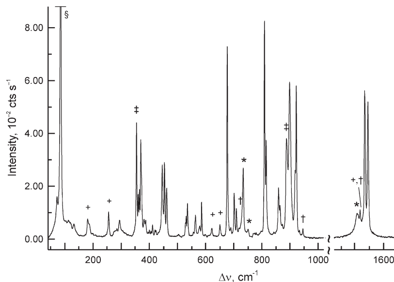
Figure 4. The Raman spectrum of [F_3S(N\equiv SF_3)_2][AsF_6] recorded at -160^\circ C using 1064-nm excitation. Symbols denote bands from unreacted [F_4S=N-Xe---N\equiv SF_3][AsF_6] (+), cis-N_2F_2 (†), coincidence of F_3S(N\equiv SF_3)_2^+ and cis-N_2F_2 bands (‡), FEP sample tube lines (*), and an instrumental artifact (S).
