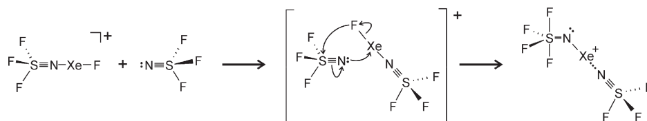
Scheme 1. Proposed Mechanism for the N≡SF 3 -Promoted Fluoride Rearrangement of F 3 S≡NXeF +
