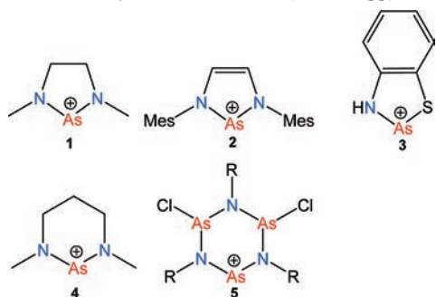
Scheme 1. Known Cyclic As–N Cations (5: R = Dipp) 7,17–20
