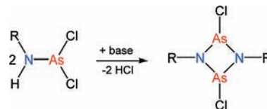
Scheme 3. Synthesis of 1,3-Dichloro- cyclo -1,3-diarsa-2,4-diazanes (6: R = Ter; 9: R = Mes*)
