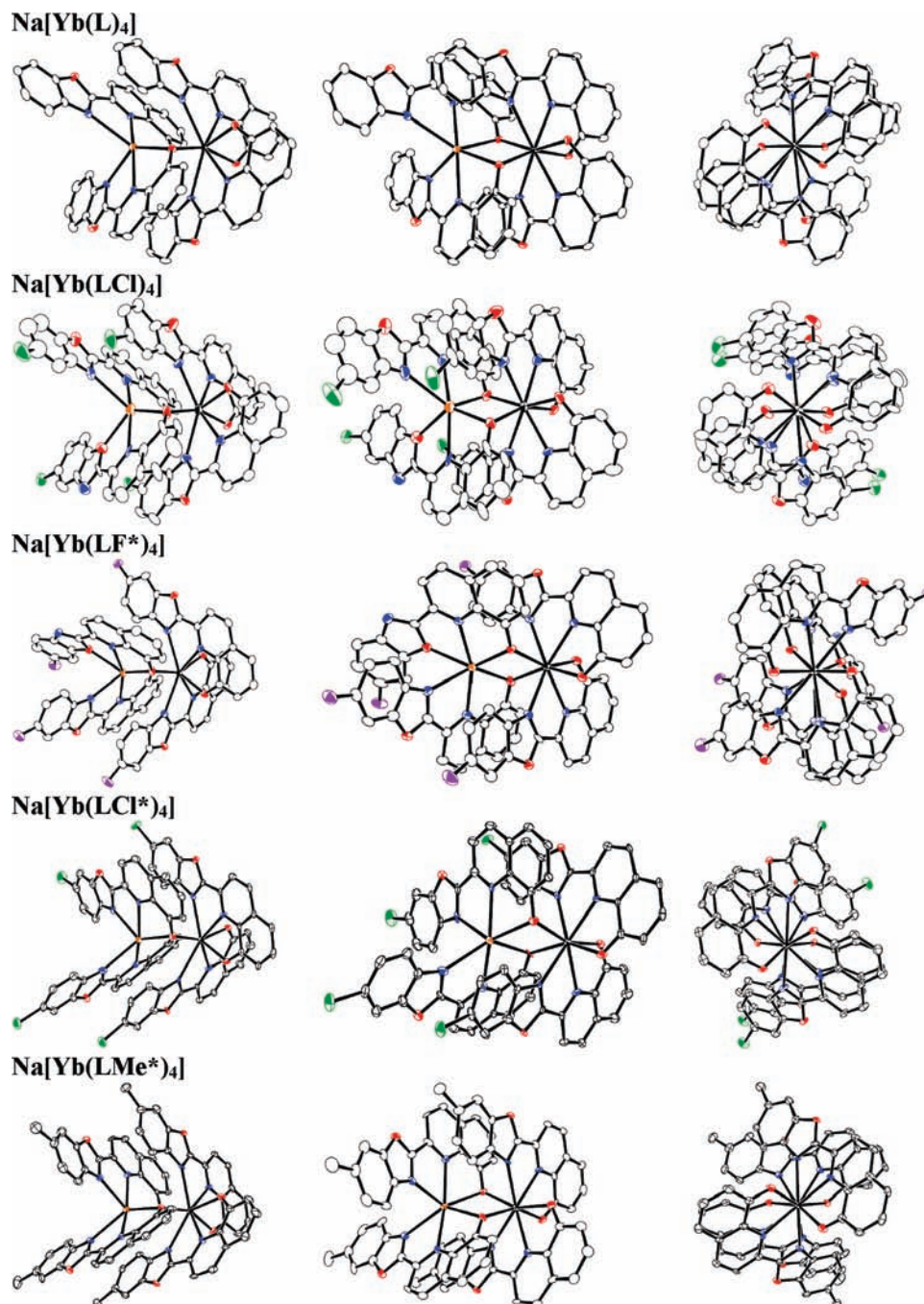
Figure 1. Molecular structures of the complexes Na[Yb(ligand) 4 ] (three views, 50% probability ellipsoids, H atoms and cocrystallized solvent molecules omitted). Heteroatoms: O, red; N, blue; F, purple; Cl, green; Yb, black; Na, orange. The idealized C 2 axis runs through Na and Yb and is in the plane of the paper (left, middle) or perpendicular to it (right).
