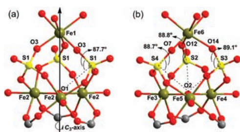
Figure 2. Two crystallographically independent tetranuclear [\text{Fe}_4(\mu_3\text{-O})(\mu_3\text{-SO}_4)_3(-\text{CO}_2)_3(\text{DMF})_6] SBUs found in 1 with (a) and without (b) 3-fold symmetry. The characteristic angles shown are compared to those in the related trinuclear [\text{Fe}_3(\mu_3\text{-O})(\mu_2\text{-SO}_4)_3(-\text{CO}_2)_3]^- SBU found in IRMOPs (see the text).
