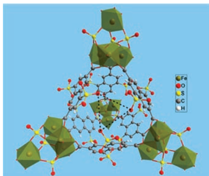
Figure 1. Molecular supertetrahedron [\text{Fe}_{16}\text{O}_4(\text{SO}_4)_{12}(\text{L}2)_6(\text{DMF})_{24}] in 1 . The size of the supertetrahedron, measured between terminal Fe atoms, is \sim 21 Å. The window aperture, defined by the three cofacial -\text{SO}_3^- groups, is indicated by the dashed regular triangle having an edge length of \sim 2 Å (excluding the van der Waals radius).
