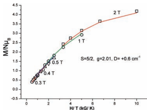
Figure 3. Plot of reduced magnetization ( M/N\mu_B ) versus H/T for 1 in the field and temperature ranges of 0.3–2 T and 2–7 K. The solid lines correspond to the fit of the data (see the SI).
