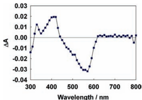
Figure 9. Nanosecond TA spectrum for the compound \text{Mo}_2(\text{OSC-2-Th})_2(\text{TiPB})_2 .
