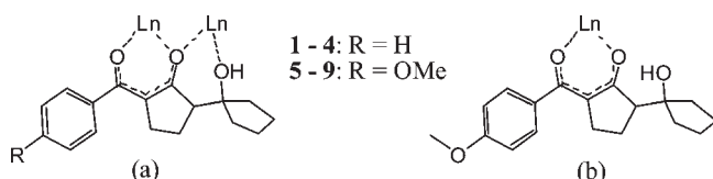
Figure 6. Coordination modes (a) \mu_2\text{-}\eta^2(\text{O},\text{O}')\eta^2(\text{O},\text{OH}) and (b) \eta^2(\text{O},\text{O}') observed in lanthanoid species reported.
