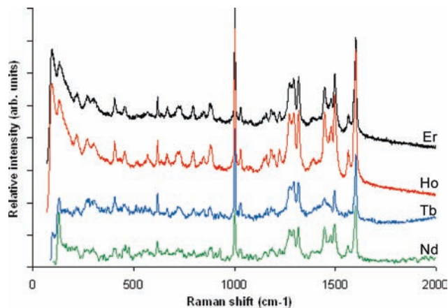
Figure 3. Raman spectra of Nd (1), Ho (2), Tb (3), and Er (4).
