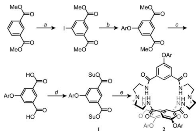
Scheme 1. Synthesis of Ligand 2 a
