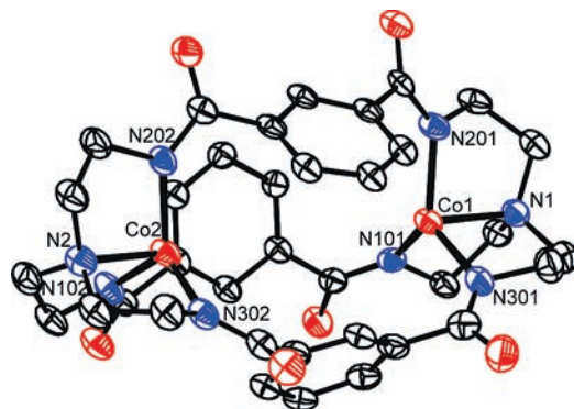
Figure 1. PLATON rendering of 3 with thermal ellipsoids drawn at 50% probability. Solvent molecules of crystallization, K + counterions, dipropoxyphenoxy groups, and H atoms are omitted for clarity.
