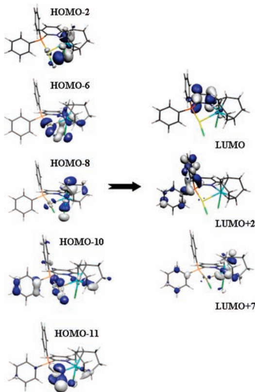
Figure 11. Relevant frontier orbitals of complex [\text{AuCl}(\text{PPh}_2\text{py})\text{Rh}(\text{cod})\text{Cl}] ( 7 ) involved in the transitions around 326 and 383 nm.
