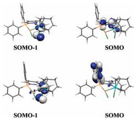
Figure 13. SOMOs in the triplet state of complexes [AuCl(PPh 2 py)-Rh(cod)Cl] ( 7 , top) and [AuCl(PPh 2 py)Ir(cod)Cl] ( 8 , bottom).
