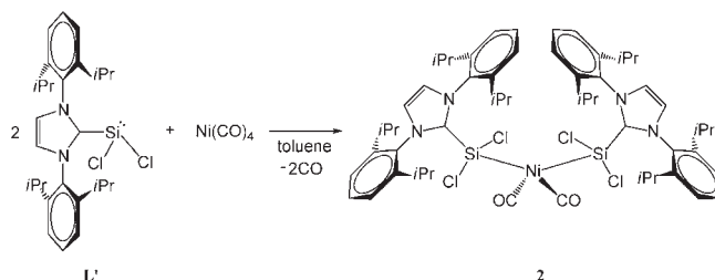
Scheme 2. Synthesis of 2
