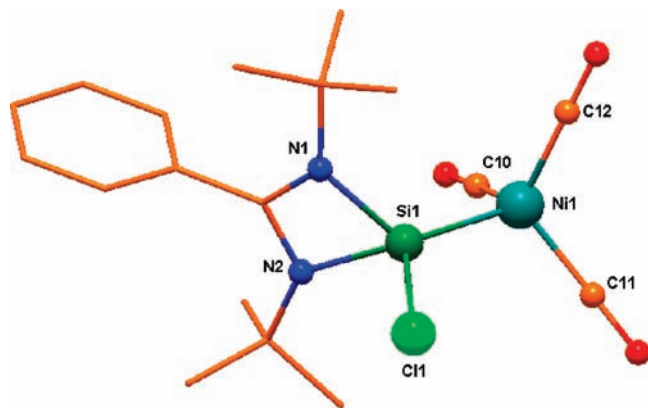
Figure 1. Crystal structure of 1 . Hydrogen atoms are omitted for clarity. Selected bond lengths (Å) and angles (deg): Ni1–Si1 2.2111(8), Ni1–C10 1.795(2), Ni1–C11 1.7967(19), Ni1–C12 1.798(2), C11–Si1 2.1149(7), Si1–N1 1.8456(15), Si1–N2 1.8373(15); C10–Ni1–C11 114.39(9), C10–Ni1–C12 114.47(9), C11–Ni1–C12 110.48(8), C10–Ni1–Si1 102.67(7), C11–Ni1–Si1 105.66(6), C12–Ni1–Si1 108.31(6), N2–Si1–N1 71.15(7), N2–Si1–C11 102.23(5), N1–Si1–C11 102.24(5), N2–Si1–Ni1 123.18(5), N1–Si1–Ni1 125.63(5), C11–Si1–Ni1 120.87(3), N2–Si1–C26 35.72(6), N1–Si1–C26 35.81(6), C11–Si1–C26 109.08(5).
