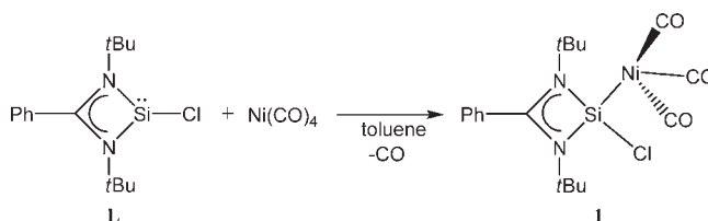
Scheme 1. Synthesis of 1
