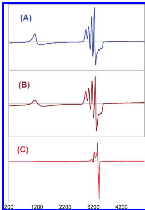
Figure 6. EPR spectra (acetone; 77 K) of (A) the product mixture of the reaction (F_8)Fe(NO)_2 + [(tmpa)Cu^I(MeCN)]^+ + 2 H^+ (blue) showing the typical heme- Fe^{III} complex and [(tmpa)Cu^{II}(solvent)]^{2+} ; (B) a madeup 1:1 mixture of [(F_8)Fe^{III}]SbF_6 and [(tmpa)Cu^I(MeCN)](ClO_4)_2 (brown); (C) the product mixture obtained from the reaction of (F_8)Fe(NO)_2 + [(tmpa)Cu^I(MeCN)]^+ in the absence of acid (red), (F_8)Fe(NO) + 1/3[(tmpa)Cu^{II}(NO_2^-)]^+ + unreacted 2/3[(tmpa)Cu^I(solvent)]^+ . See Figure S8 (Supporting Information) for an expanded view of this spectrum. See the text for further explanation.
