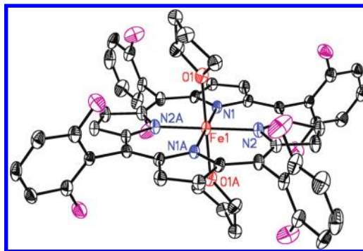
Figure 7. ORTEP diagram showing the cationic portion of [(\text{F}_8)\text{Fe}^{\text{III}}(\text{THF})_2]\text{SbF}_6 . Also see Table 4 for structural parameters.
