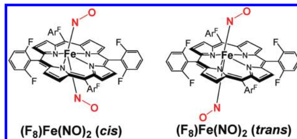
Figure 5. Two possible conformations (cis, trans) of the present (\text{F}_8)\text{Fe}(\text{NO})_2 complex. Both have been suggested, but DFT calculations in 2003 from the groups of both Ford 58 and Ghosh 59,60 support the view that the cis configuration would be the preferred structure in a porphyrinate-iron environment.
