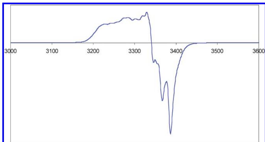
Figure 2. EPR spectrum of (THF)(F_8)Fe(NO) recorded at 77 K in THF with g_1 = 2.100, g_2 = 2.063, and g_3 = 2.011 . It is essentially identical to the spectrum of (THF)(PPDME)Fe(NO) , reported by Yoshimura. 42
