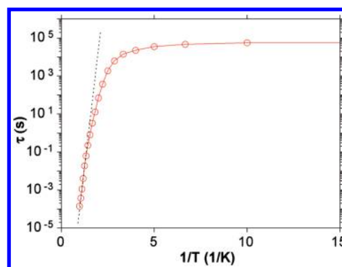
Figure 9. Arrhenius plot of the relaxation time ( \tau ) versus 1/T for a single crystal of 2 \cdot 3\text{CH}_2\text{Cl}_2 . The dashed line is the fit of the data in the thermally activated region to the Arrhenius equation; see the text for the fit parameters.
