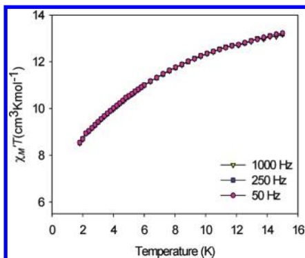
Figure 4. In-phase ac susceptibility ( \chi_M' ) signal, plotted as \chi_M' T versus T , for complex 1 \cdot \text{MeCN} in a 3.5 G field oscillating at the indicated frequencies.
