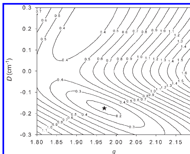
Figure 6. Two-dimensional contour plot of the root-mean-square error surface for the D versus g fit for complex 2 \cdot 3\text{H}_2\text{O} . The star marks the best-fit position.
