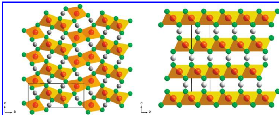
Figure 1. Polyhedral projections of the crystal structures of \alpha -SrNCN (left) and \beta -SrNCN (right) with the SrN 6 octahedra given in orange, Sr atoms in red, N atoms in green, and C atoms in gray.
