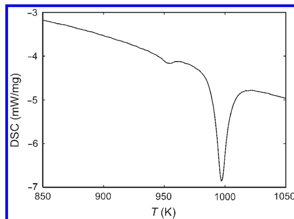
Figure 7. DSC of \beta -SrNCN in going from T = 850 – 1050 K; see also text.
