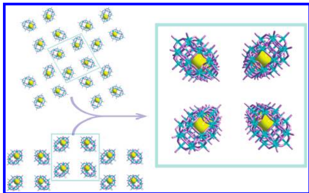
Figure 2. Representations of the packing mode of 1 : \beta -[H 2 W 18 O 57 (SO 3 ) 6- ]. Above : view along the 4-fold axis; below : side view of the 4-fold axis showing polar packing of the cluster. The {W 18 } cage is shown in wire mode and each cyan line represents one W center. The S atoms are shown by the yellow spheres and the O ligands are depicted by the pink colored sticks.
