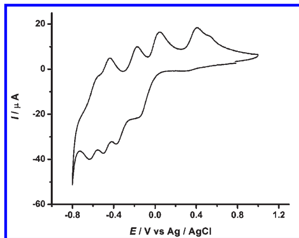
Figure 7. Cyclic voltammogram of compound 2 ( 2 \times 10^{-3} M) in aqueous 0.2 M \text{Na}_2\text{SO}_4 of 1 M \text{CH}_3\text{COOH}/\text{CH}_3\text{COONa} buffer solution (pH = 4.2). The scan rate was 100 \text{ mV s}^{-1} , the working electrode was glassy carbon (1.5 mm), and the reference electrode was Ag/AgCl.
