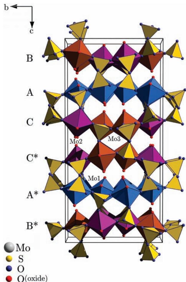
Figure 6. The three different types of layers (A, B, C) in \text{MoO}_2(\text{SO}_4) connected to a three-dimensional network. Layers of type A contain only [\text{Mo1O}_2] units (blue), whereas B and C are built by both [\text{Mo2O}_2] (violet) and [\text{Mo3O}_2] (brown). The layers A*, B*, and C* are generated by glide planes located at z = 0, 0.5, and 1 . Along [100] , channels are formed, which accommodate one-half of the terminal oxide ligands on each Mo atom.
