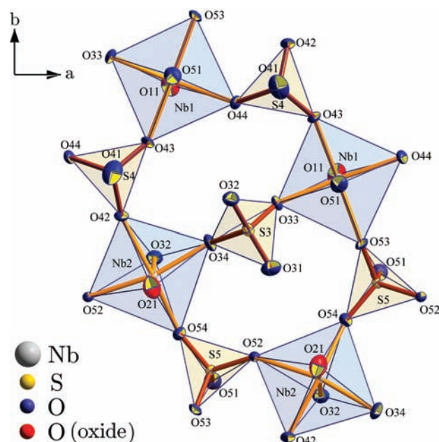
Figure 1. Atom labeling scheme and thermal ellipsoids drawn at 75% probability for \text{Nb}_2\text{O}_2(\text{SO}_4)_3 . Four [\text{Nb}=\text{O}] units are connected through four [\text{SO}_4] tetrahedra to eight-membered rings, which are centered by an additional sulfate group. For both crystallographically distinguishable Nb atoms, a distorted octahedral coordination results.
