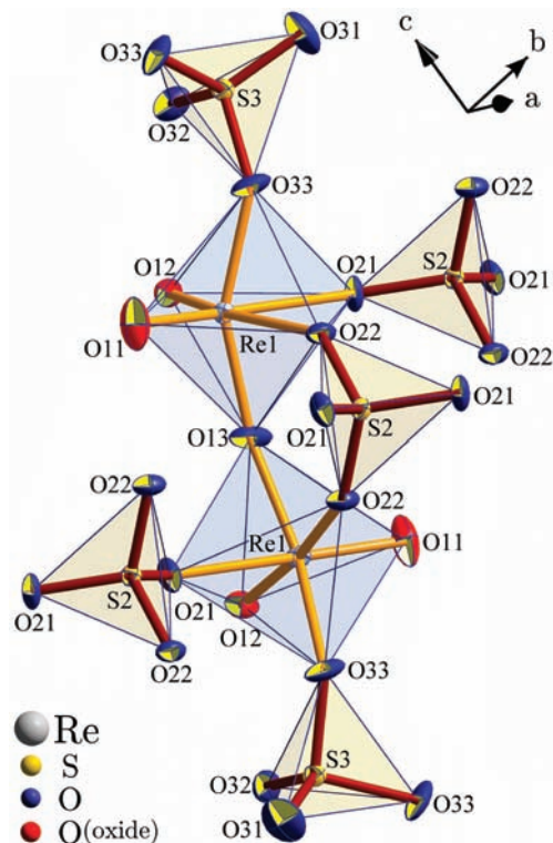
Figure 13. Atom labeling scheme and thermal ellipsoids drawn at a 75% probability level for \text{Re}_2\text{O}_5(\text{SO}_4)_2\text{-II} . Each Re atom is in distorted octahedral coordination with two terminal oxide ligands, one bridging oxygen atom, and three sulfate ions. In the [\text{Re}_2\text{O}_5] unit formed, the tilt of the [\text{ReO}_2] moieties is much more pronounced than in \text{Re}_2\text{O}_5(\text{SO}_4)_2\text{-I} .
