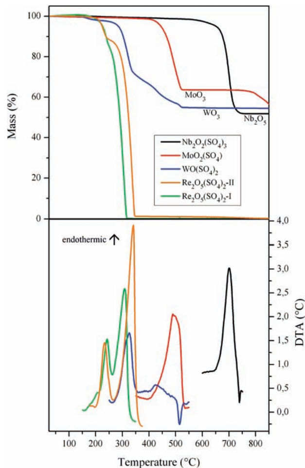
Figure 16. Results of the thermogravimetric measurements (top) and differential thermal analysis (below) for \text{Nb}_2\text{O}_2(\text{SO}_4)_3 , \text{MoO}_2(\text{SO}_4) , \text{WO}(\text{SO}_4)_2 , and \text{Re}_2\text{O}_5(\text{SO}_4)_2\text{-I} and \text{-II} . For clarity reasons, only the relevant parts of the DTA curves are plotted. The full graphs are available as Supporting Information.
