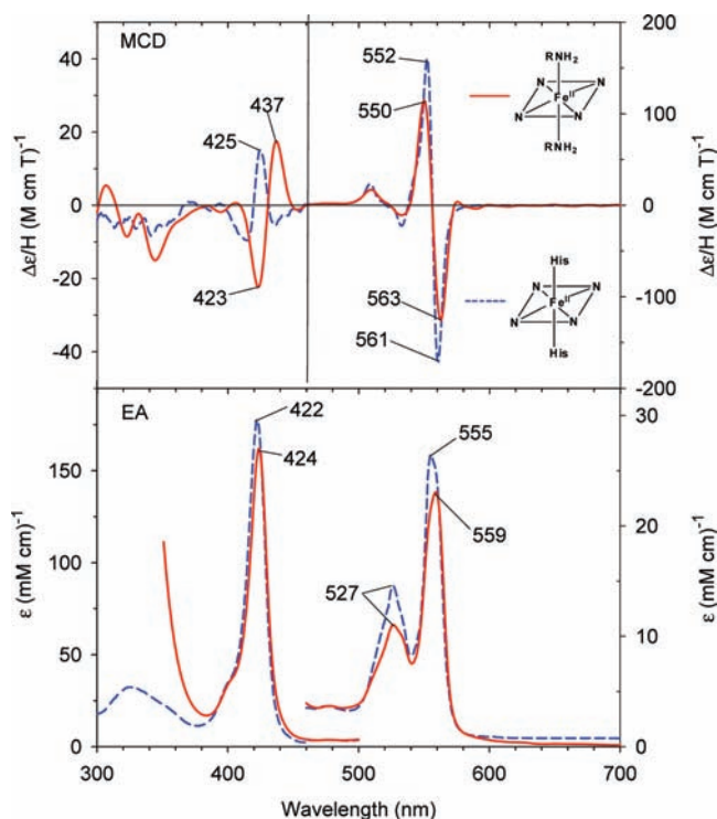
Figure 7. MCD (top) and electronic absorption (bottom) spectra of the deoxyferrous H93G(bis-methylamine) Mb (144 mM methylamine; solid line) compared to previously reported deoxyferrous cytochrome b 5 (dashed line). 40 The spectra were recorded in 0.1 M potassium phosphate at pH 7.0 at 4 °C.
