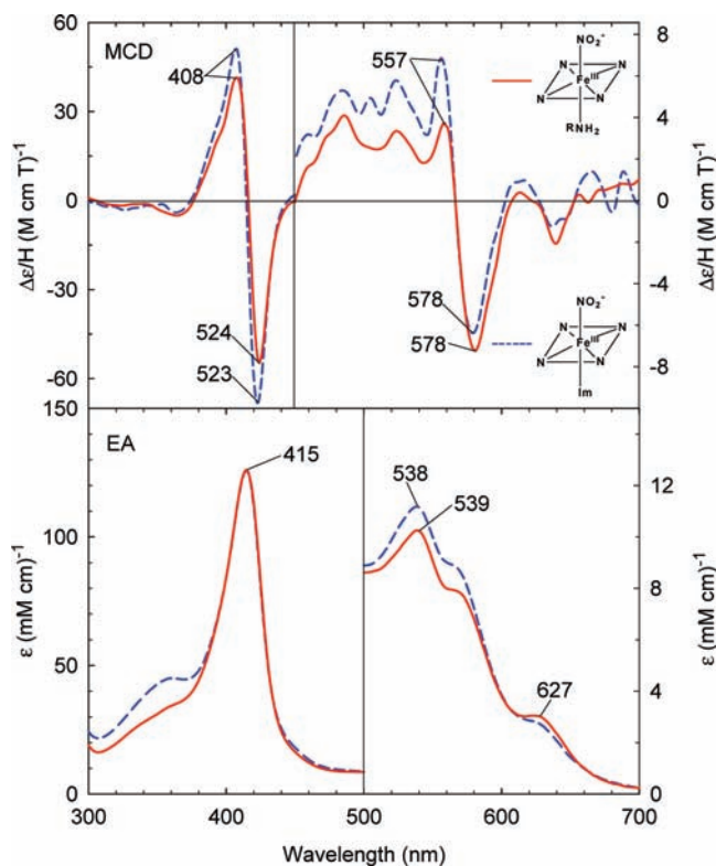
Figure 4. MCD (top) and electronic absorption (bottom) spectra of cyclohexylamine and nitrite (NO 2 )-bound ferric H93G Mb (0.5 M cyclohexylamine, 0.1 M NaNO 2 ; solid line) compared to 4-methylimidazole (4Me-Im) and nitrite (NO 2 )-bound ferric H93G Mb (0.1 mM 4Me-Im, 0.1 M NaNO 2 ; dashed line). The spectra were recorded in 0.1 M potassium phosphate at pH 7.0 at 4 °C.
