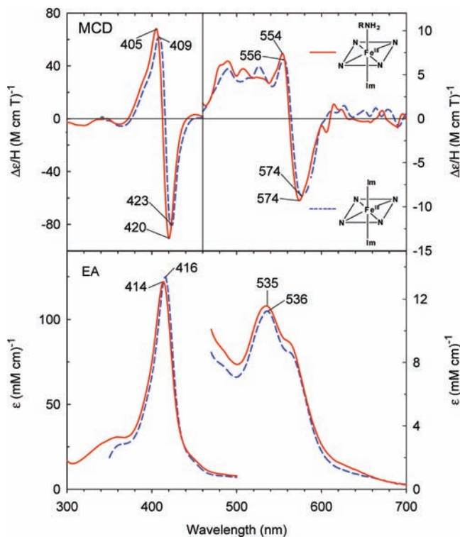
Figure 5. MCD (top) and electronic absorption (bottom) spectra of cyclohexylamine and Im-bound ferric H93G Mb (0.2 mM Im, 1 M cyclohexylamine; solid line) compared to previously reported bis-Im-bound ferric H93G(Im) Mb (2 M Im; dashed line). 28 The spectra were recorded in 0.1 M potassium phosphate at pH 7.0 at 4 °C.
