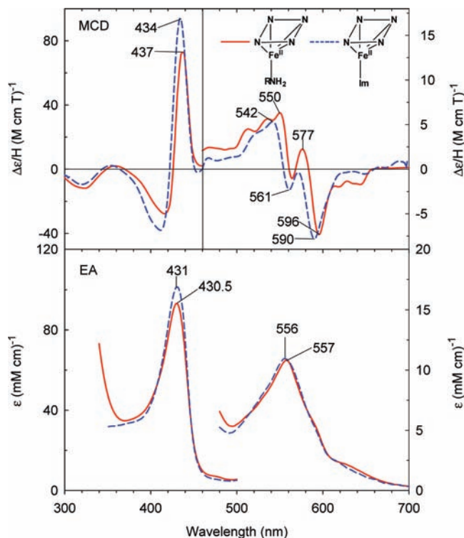
Figure 6. MCD (top) and electronic absorption (bottom) spectra of the deoxyferrous H93G(cyclohexylamine) Mb (0.3 M cyclohexylamine; solid line) compared to previously reported deoxyferrous H93G(Im) Mb (1 mM Im; dashed line). 27 The spectra were recorded in 0.1 M potassium phosphate at pH 7.0 at 4 °C.
