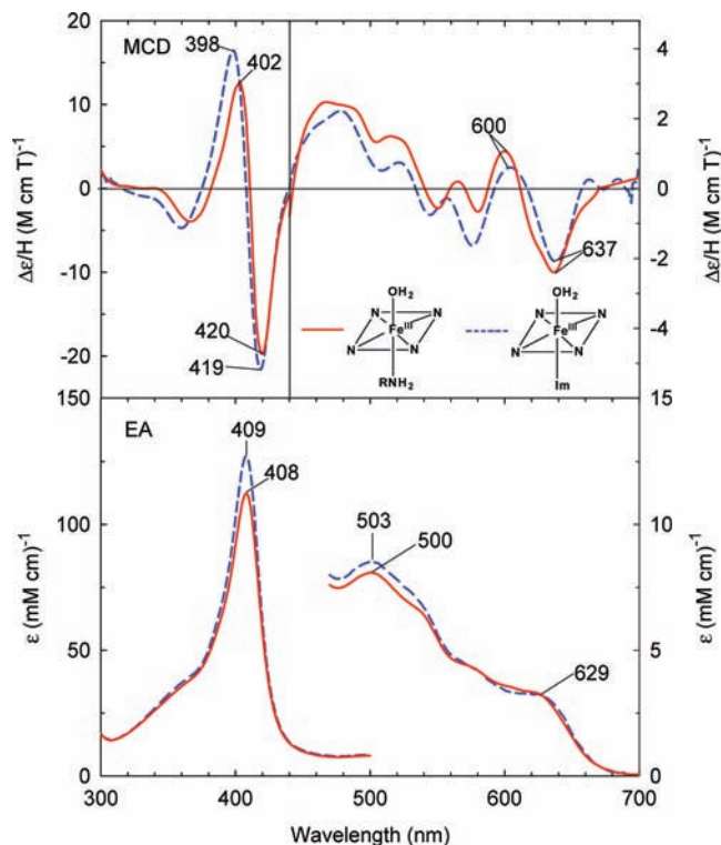
Figure 2. MCD (top) and electronic absorption (bottom) spectra of ferric H93G(cyclohexylamine) Mb (0.3 M cyclohexylamine; solid line) compared to previously reported ferric H93G(Im) Mb (1 mM Im; dashed line). 27 The spectra were recorded in 0.1 M potassium phosphate at pH 7.0 at 4 °C.
