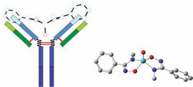
Figure 7. ^{99m}\text{Tc} -labeled N -substituted BHAM as an IgG antibody mimic. The Y-like shaped structure of ^{99m}\text{Tc} -MBHAM suggests that when a targeting molecule is incorporated via each amine group in BHAM, the two targeting molecules would point to each direction of the two heavy chains of an IgG antibody.
