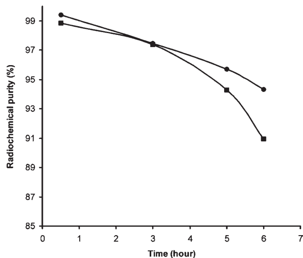
Figure 4. Percent radiochemical purity of ^{99m}\text{Tc} -BHAM (■) and ^{99m}\text{Tc} -MBHAM (●) as a function of time when the ligand concentration was fixed at 10^{-5} M.
