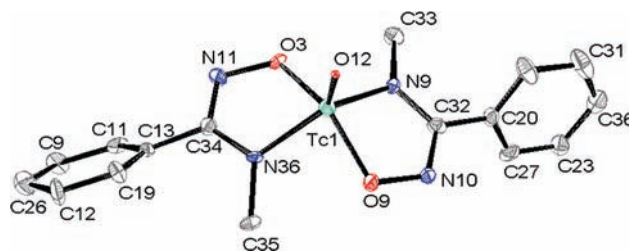
Figure 5. Molecular structure of ^{99g}\text{Tc} -MBHAM with atom-labeling scheme. Hydrogen atoms are omitted for clarity.
