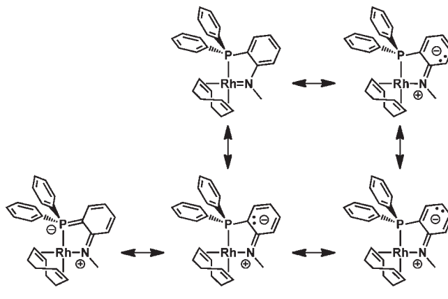
Scheme 2. Possible Resonance Description of Compound 1a
