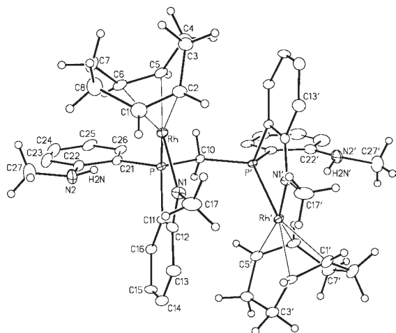
Figure 2. ORTEP Diagram of [\text{Rh}_2(\text{COD})_2(\mu\text{-P,N,P',N'-mapm}^{2-})] (2). Thermal ellipsoids as in Figure 1. Hydrogen atoms are shown with arbitrarily small thermal parameters for the cyclooctadiene, methyl, methylene, and amine groups, and are not shown for the aryl rings.
