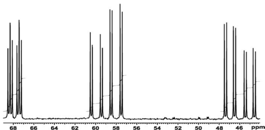
Figure 3. ^{31}\text{P}\{^1\text{H}\} NMR Spectrum of [\text{Rh}(\text{P},\text{P}'\text{-dppe})(\text{P},\text{N}\text{-Ph}_2\text{PAr}^-)] (3).
