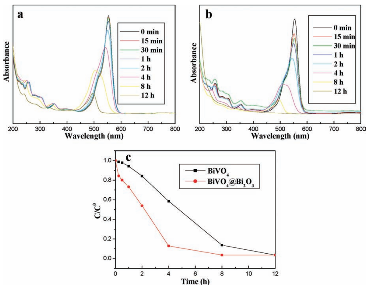
Figure 6. Changes of UV-vis spectra of olive-shaped \text{BiVO}_4 (a) and core-shell \text{BiVO}_4@ \text{Bi}_2\text{O}_3 microspheres (b) suspended in a RhB solution as a function of the irradiation time and RhB concentration changes over olive-shaped \text{BiVO}_4 and core-shell \text{BiVO}_4@ \text{Bi}_2\text{O}_3 microspheres (c), respectively.
