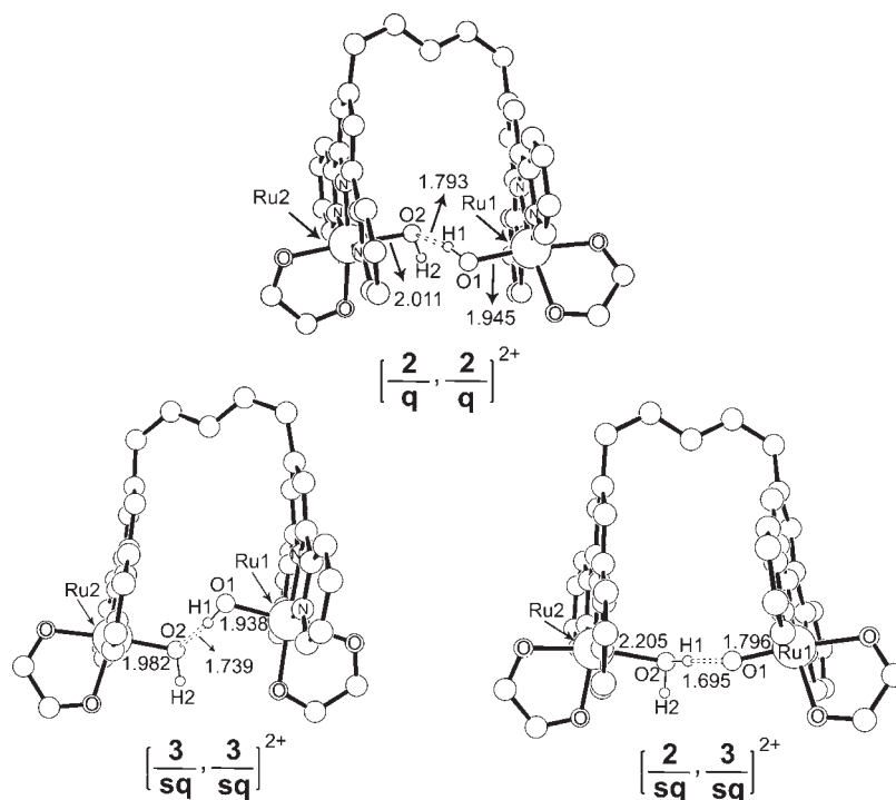
Figure 3. Structures of the alternative candidates for the ground electronic state of [2,2]^{2+} . Only the core structures are shown for clarity; only a few selected carbon atoms of the anthracene and the quinone fragments are drawn, and all nonessential hydrogen atoms are hidden.
