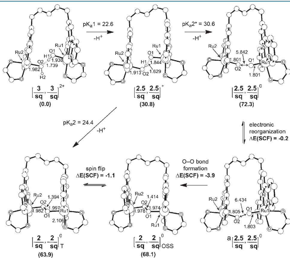
Figure 4. Structures of the intermediates during the deprotonation process in methanol. Solution-phase free energies in kcal mol -1 are given in parentheses. Electronic energy differences \Delta E(\text{SCF}) are also in kcal mol -1 .
