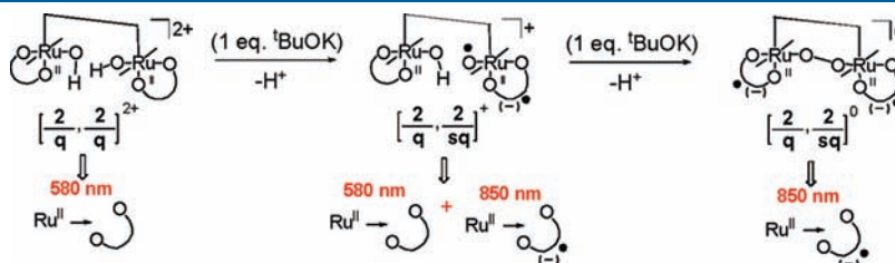
Figure 2. Tanaka's proposal for the deprotonation process in methanol in the presence of {}^t\text{BuOK} .
