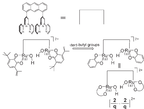
Figure 1. Computational model, and abbreviations used in this study.
