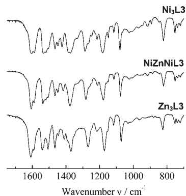
Figure 2. FT-IR spectra of the homo- and heterotrinnuclear complexes.
