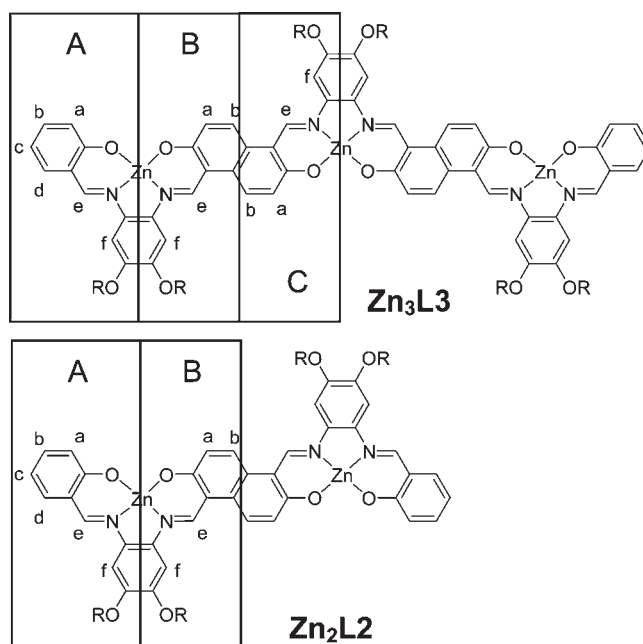
Figure 1. Comparison of di- and trinuclear complexes for ^1\text{H} NMR analysis.
