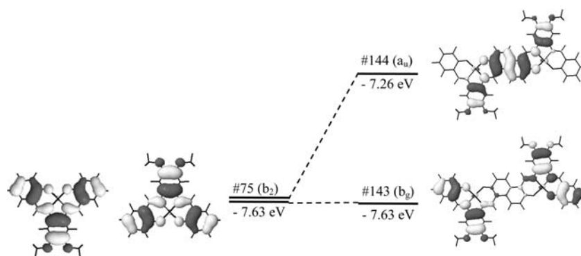
Figure 4. Schematic representation of interorbital interaction that generates near-HOMO orbitals of Ni 2 L 2 .
