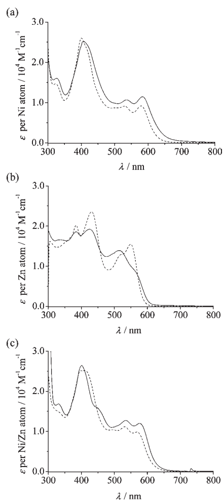
Figure 3. UV-vis absorption spectra of trinuclear (solid line) and dinuclear (dashed line) complexes: (a) \text{Ni}_3\text{L}_3 and \text{Ni}_2\text{L}_2 , (b) \text{Zn}_3\text{L}_3 and \text{Zn}_2\text{L}_2 , and (c) \text{NiZnNiL}_3 and \text{NiZnL}_2 . Absorption coefficients are normalized by the number of metal atoms per molecule.
