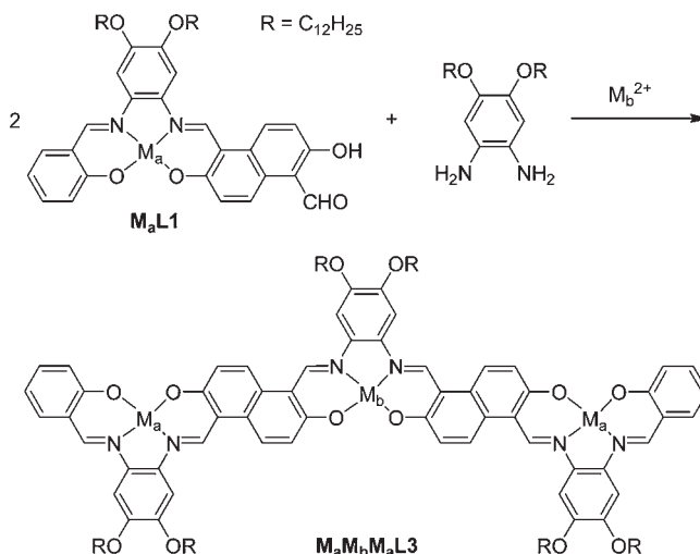
Scheme 1. Synthesis of the Trinuclear Complex M_aM_bM_aL3
