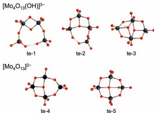
Figure 7. Ball-and-stick representations for the optimized structures of the most representative tetranuclear species with [\text{Mo}_4\text{O}_{13}(\text{OH})]^{3-} (te-1, te-2, and te-3) and [\text{Mo}_4\text{O}_{13}]^{2-} (te-4 and te-5) stoichiometries.
