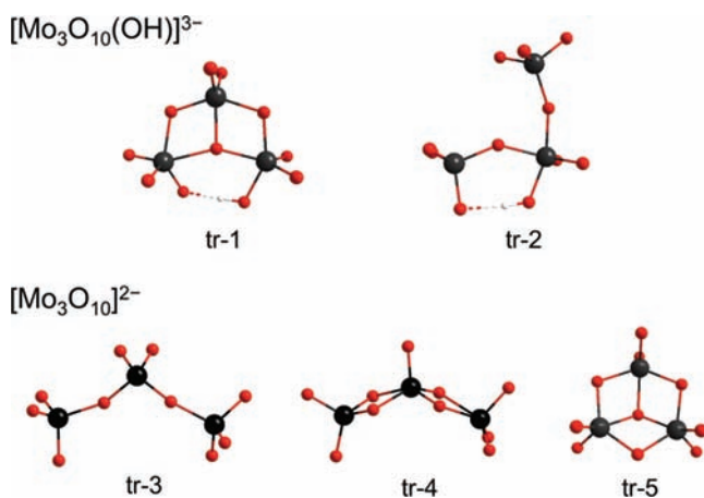
Figure 6. Ball-and-stick representations for the optimized structures of the most representative trinuclear species with [\text{Mo}_3\text{O}_{10}(\text{OH})]^{3-} (tr-1 and tr-2) and [\text{Mo}_3\text{O}_{10}]^{2-} (tr-3, tr-4 and tr-5) stoichiometries.
