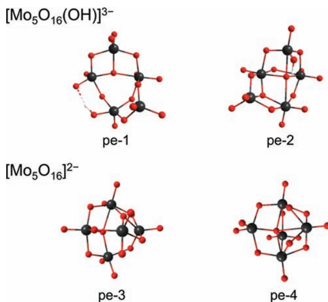
Figure 8. Ball-and-stick representations for the optimized structures of the most representative pentanuclear species with [\text{Mo}_5\text{O}_{16}(\text{OH})]^{3-} (pe-1, pe-2) and [\text{Mo}_5\text{O}_{16}]^{2-} (pe-3 and pe-4) stoichiometries.
