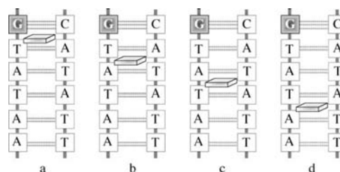
Figure 6. Schematization of the possible situations (see text). The intercalated 1 is shown as a perpendicular object. The guanine quencher units are highlighted in gray.
