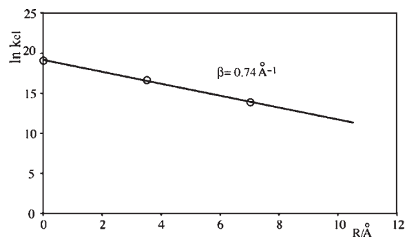
Figure 7. Distance dependence of \ln k_{\text{et}} , according to eq 1.
