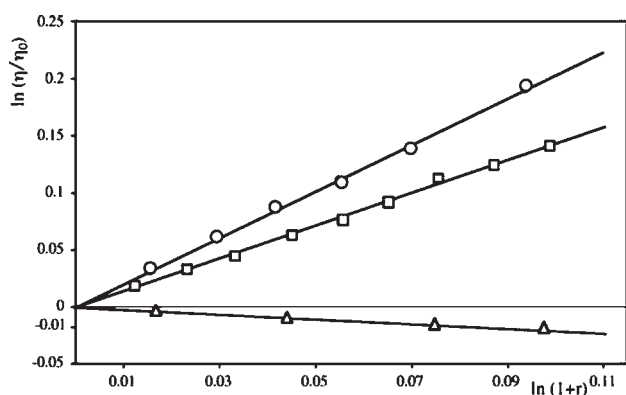
Figure 3. Viscometric titrations of calf-thymus DNA solutions ( 6.0 \times 10^{-4} M) with [\text{Ru}(\text{bpy})_2(\text{dppz})]^{2+} (○), 1 (□), and 2 (△) at 25 °C and pH 7 ( 1 \times 10^{-3} M phosphate buffer, and 1.0 \times 10^{-2} M NaCl). \eta_0 = reduced viscosity of the DNA solution; \eta = reduced viscosity of the DNA solution in the presence of compounds; r = [\text{compound}]_{\text{bound}}/[\text{DNA}]_{\text{tot}} .
