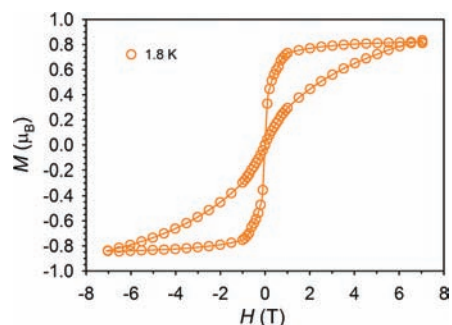
Figure 4. Variable-field magnetization data for the 1:1 diluted compound \text{U}_{0.5}\text{Y}_{0.5}(\text{H}_2\text{BPz}_2)_3 . The solid line serves as a guide for the eye.
