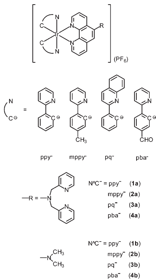
Chart 1. Structures of the Iridium(III) Complexes
