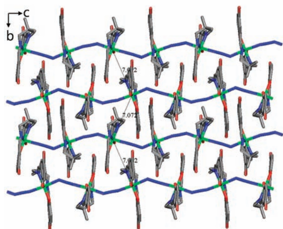
Figure 3. Top: Crystal structure of 3 showing the atom-labeling schemes. Symmetry codes: e, x, 1.5 - y, 0.5 + z ; f, x, 1.5 - y, -0.5 + z . Bottom: Extended 2D view with the shortest interchain distance (dotted lines).
