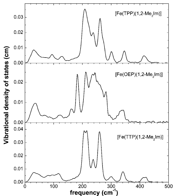
Figure 2. Experimental NRVS spectra of polycrystalline (powder) samples of 1,2-dimethylimidazole-ligated species. [Fe(TPP)(1,2-Me 2 Im)] (microcrystalline, upper panel), [Fe(OEP)(1,2-Me 2 Im)] (microcrystalline, center panel), [Fe(TTP)(1,2-Me 2 Im)] (microcrystalline, lower panel).
