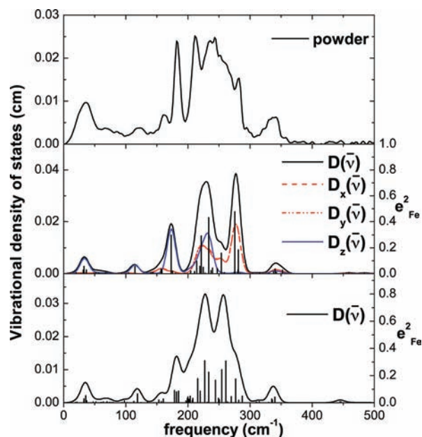
Figure 9. Comparison of the experimental VDOS determined from NRVS measurements on [\text{Fe}(\text{OEP})(1,2\text{-Me}_2\text{Im})] (upper panel) with the DFT-predicted VDOS from DFT calculations using the observed conformation of the peripheral ethyl groups (center panel, four up and four down) and an energy minimized conformation (lower panel, alternating two up, two down).
