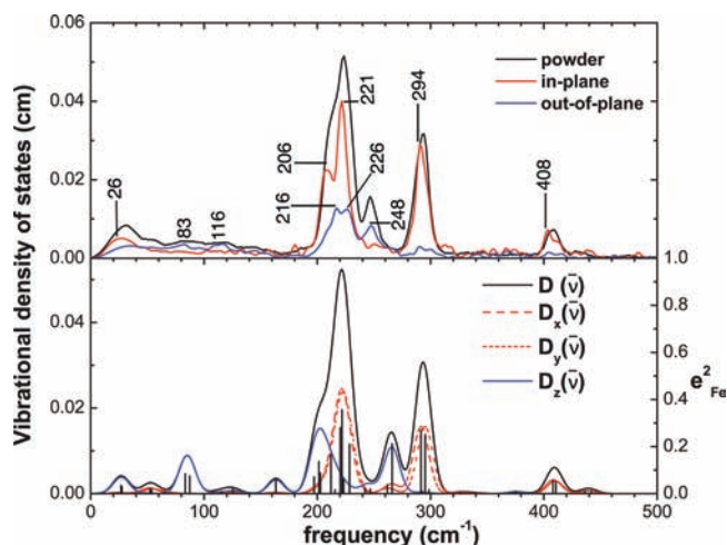
Figure 3. Comparison of the experimental VDOS determined from NRVs measurements on [\text{Fe}(\text{TPP})(2\text{-MeHIm})] (upper panel) with the DFT-predicted VDOS on (lower panel). The spectra in the top panel have been normalized so that the following relationship is followed: D(\bar{\nu}) = 2D_{\text{ip}}(\bar{\nu}) + D_{\text{oop}}(\bar{\nu}) .
