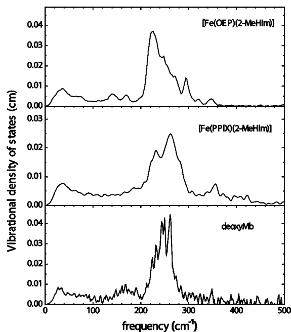
Figure 10. Comparison of the experimental VDOS determined from NRVS measurements on [\text{Fe}(\text{OEP})(2\text{-MeHIm})] (upper panel) with [\text{Fe}(\text{PPIX})(2\text{-MeHIm})] (center panel) and deoxyMb (lower panel).
