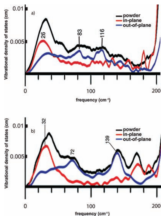
Figure 11. Expanded view of the 0–200 \text{cm}^{-1} region for (top) [\text{Fe}(\text{TPP})(2\text{-MeHIm})] and (bottom) that for [\text{Fe}(\text{OEP})(2\text{-MeHIm})] .
