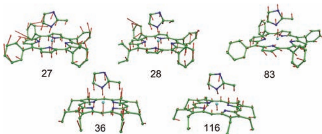
Figure 12. Predicted oop modes at 27, 28, and 83 \text{cm}^{-1} for [\text{Fe}(\text{TPP})(2\text{-MeHIm})] (top); the predicted mode at 87 \text{cm}^{-1} is similar to the 83 \text{cm}^{-1} mode. Predicted out-of-plane modes at 36 and 116 \text{cm}^{-1} for [\text{Fe}(\text{OEP})(2\text{-MeHIm})] (bottom).
