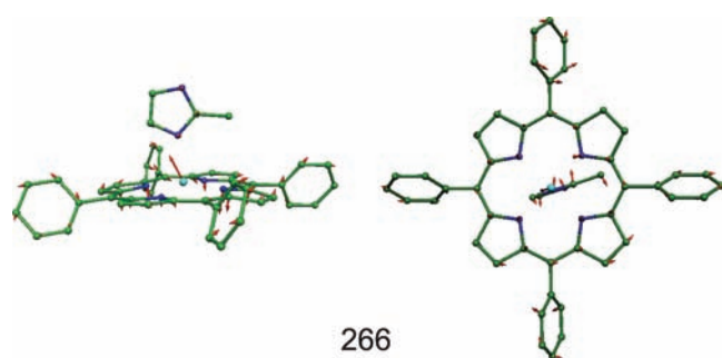
Figure 8. Out-of-plane Fe mode, predicted at 266 \text{cm}^{-1} , contributing to the experimental feature at 248 \text{cm}^{-1} in [\text{Fe}(\text{TPP})(2\text{-MeHIm})] .
