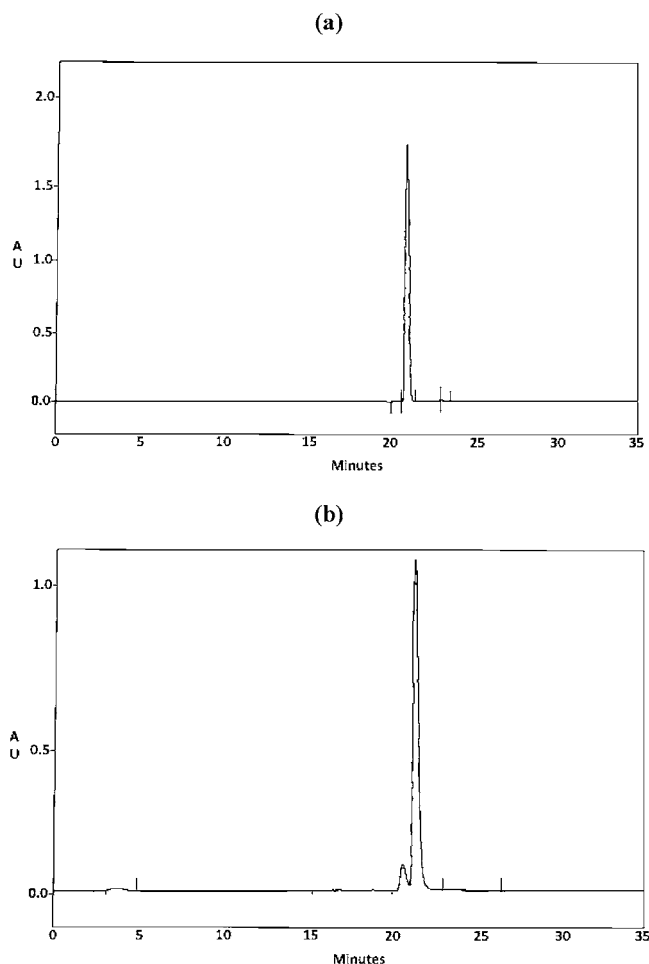
Figure 1. HPLC chromatograms of (a) syn -[Re(N)(SNS)(PPh 3 )] (2) and (b) a mixture of syn/anti -[ 99 Tc(N)(SNS)(PPh 3 )] (1).
