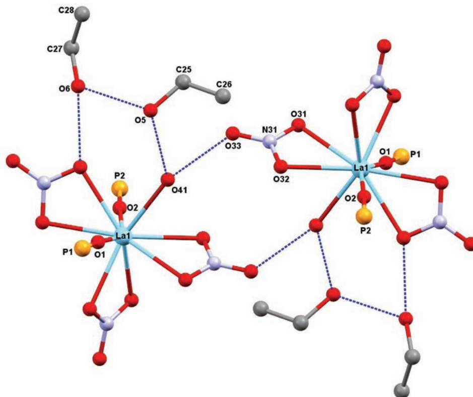
Figure 5. Hydrogen bonding network in \text{La}(\text{NO}_3)_3(\text{tBu}_3\text{PO})_2\text{H}_2\text{O}\cdot 2\text{EtOH} ( 1 ) (tBu groups and all hydrogen atoms have been omitted for clarity). \text{O5}-\text{H5}\cdots\text{O6}^i = 2.727(4) Å, \text{O6}-\text{H6}\cdots\text{O12}^{ii} = 2.838(4) Å, \text{O41}-\text{H42}\cdots\text{O33}^{iii} = 2.907(4) Å, \text{O41}-\text{H41}\cdots\text{O5} = 2.718(4) Å; Symmetry transformations used to generate equivalent atoms: (i) -x + 3/2, y + 1/2, -z + 3/2 , (ii) -x + 3/2, y - 1/2, -z + 3/2 , (iii) -x + 1, -y + 1, -z + 2 .
