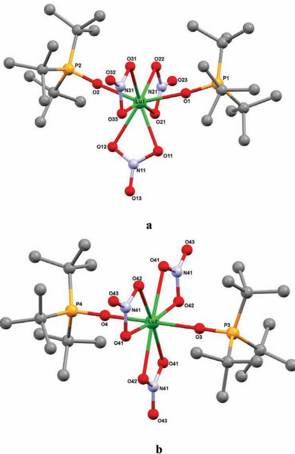
Figure 3. Molecular structures of the two isomers of \text{Lu}(\text{NO}_3)_3(\text{tBu}_3\text{PO})_2 ( 7 ); a ) the 70% isomer, b ) the 30% isomer (H atoms have been omitted for clarity).
