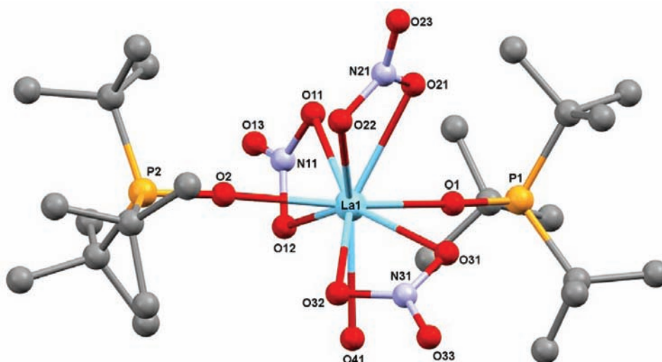
Figure 1. Molecular structure of \text{La}(\text{NO}_3)_3(\text{tBu}_3\text{PO})_2 \cdot \text{H}_2\text{O} \cdot 2\text{EtOH} (1) (H atoms and the lattice ethanol molecules have been omitted for clarity).
