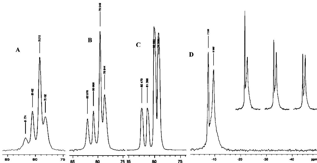
Figure 6. CPMAS ^{31}\text{P} and ^{15}\text{N} NMR spectra of \text{Lu}(\text{NO}_3)_3(\text{tBu}_3\text{PO})_4 .
