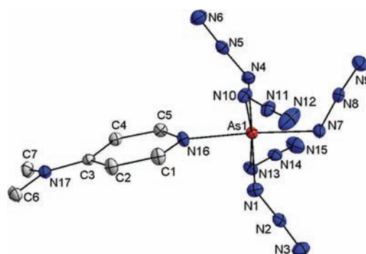
Figure 2. Representation of dmap- As(N_3)_5 1 (hydrogen atoms omitted for clarity, thermal ellipsoids at 50% probability levels). Bond lengths [Å] and angles [°]: As1–N1 1.9233(13), As1–N4 1.9291(13), As1–N7 1.9348(13), As1–N10 1.9268(13), As1–N13 1.9238(12), As1–N16 1.9846(12), N1–N2 1.2338(18), N2–N3 1.1310(19), N7–N8 1.2290(18), N8–N9 1.1297(19); N1–As1–N4 179.59(6), N7–As1–N16 175.78(5), N13–As1–N10 172.97(5), N1–As1–N13 90.12(5), N1–As1–N10 90.32(6), N13–As1–N4 90.03(5), N10–As1–N4 89.48(6), N1–As1–N7 90.02(6), N13–As1–N7 90.14(6), N10–As1–N7 96.87(6), N4–As1–N7 90.36(6), N1–As1–N16 88.33(6), N13–As1–N16 85.98(5), N10–As1–N16 87.02(5), N4–As1–N16 91.31(5), N2–N1–As1 113.07(10), N14–N13–As1 115.76(10), N3–N2–N1 175.85(15), N9–N8–N7 174.89(16).
