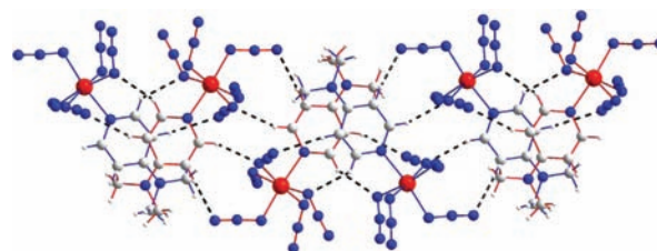
Figure 4. Chain formation parallel to the a axis via CH...N in the packing of 2 . The bonds of the independent molecules of the asymmetric unit are displayed in different colors (red, blue), hydrogen bond in dashed lines.
