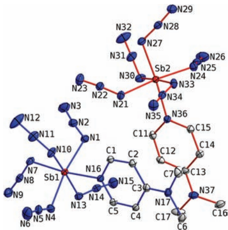
Figure 3. Asymmetric unit of dmap-Sb(N 3 ) 5 2 consisting of two independent molecules (one depicted with red bond lines the other with blue ones; hydrogen atoms omitted for clarity, thermal ellipsoids at 50% probability levels). Bond lengths [Å] and angles [°] of one independent molecule (displayed with blue bonds): Sb1–N1 2.0814(12), Sb1–N4 2.0636(12), Sb1–N7 2.0716(12), Sb1–N10 2.0751(12), Sb1–N13 2.0726(13), Sb1–N16 2.1366(11), N1–N2 1.2311(19), N2–N3 1.1316(19), N7–N8 1.2255(18), N8–N9 1.1319(19); N1–Sb1–N4 170.25(5), N13–Sb1–N10 171.93(5), N7–Sb1–N16 172.95(5), N4–Sb1–N7 95.64(5), N4–Sb1–N13 79.79(5), N7–Sb1–N13 95.16(5), N4–Sb1–N10 93.63(5), N7–Sb1–N10 90.10(5), N7–Sb1–N1 91.73(5), N13–Sb1–N1 93.21(5), N10–Sb1–N1 92.74(5), N4–Sb1–N16 89.80(5), N13–Sb1–N16 90.21(5), N10–Sb1–N16 85.06(5), N1–Sb1–N16 83.40(5), Sb1–N1–N2 118.72(10), Sb1–N13–N14 119.67(10), N1–N2–N3 174.47(17), N7–N8–N9 175.68(15). The geometrical parameters of the second molecule are similar and can be found in the Supporting Information.
