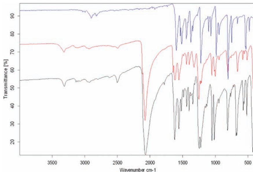
Figure 1. IR spectra of dmap- E(N_3)_5 ( E = As 1 (black), Sb 2 (red)) and dmap (blue).
