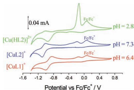
Figure 5. Cyclic voltammograms (scan rate 150 mV/s) of [CuL1] + and [CuL2] + recorded at different pH values.
